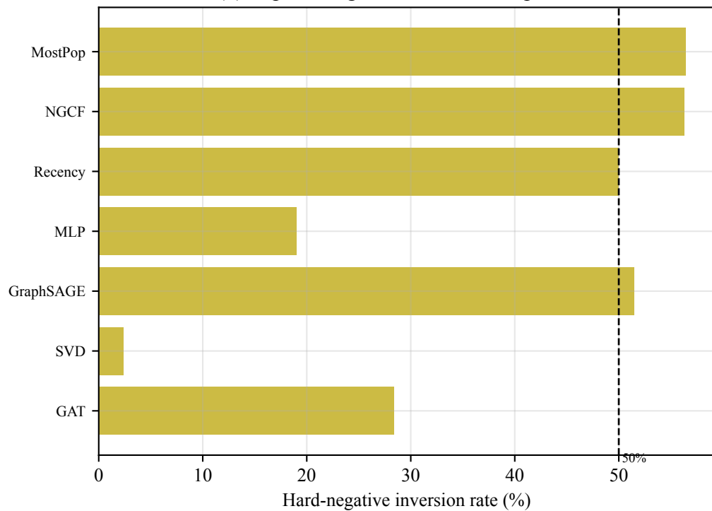
(b) Popular negatives outrank the positive
