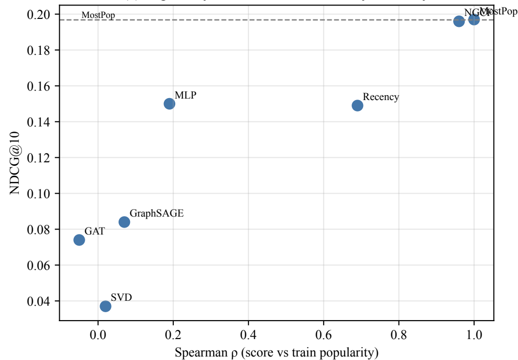
(a) Popularity correlation does not buy accuracy
