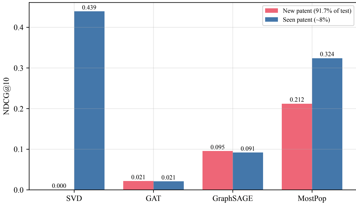
Patent cold-start: SVD scores 0.000 on unseen patents
