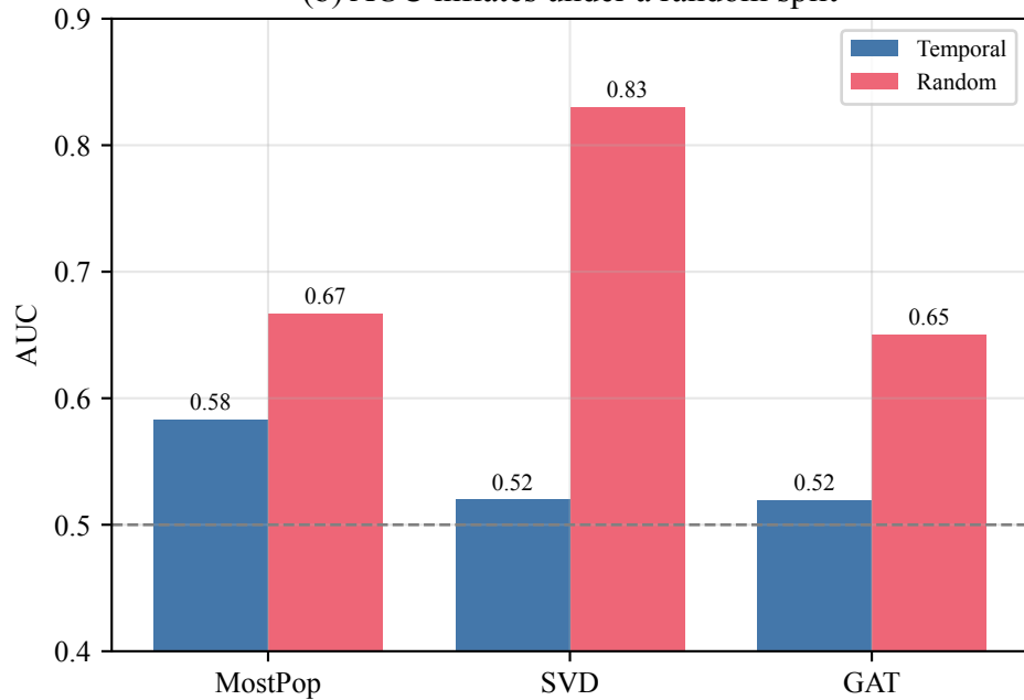
(b) AUC inflates under a random split
