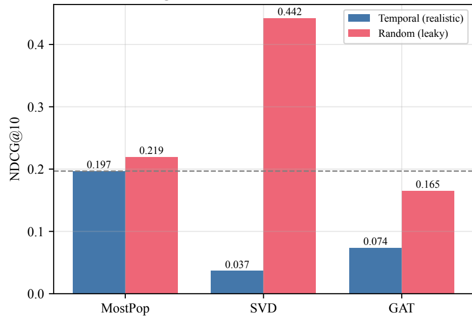
(a) NDCG@10: SVD wins only under a random split
