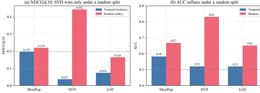
Figure 8: RQ1: temporal vs. random split. A random split lowers the cold-start rate (91.7%→2.4%) and reverses the verdict — (a) SVD becomes the best model by NDCG@10, and (b) AUC inflates across the board.
