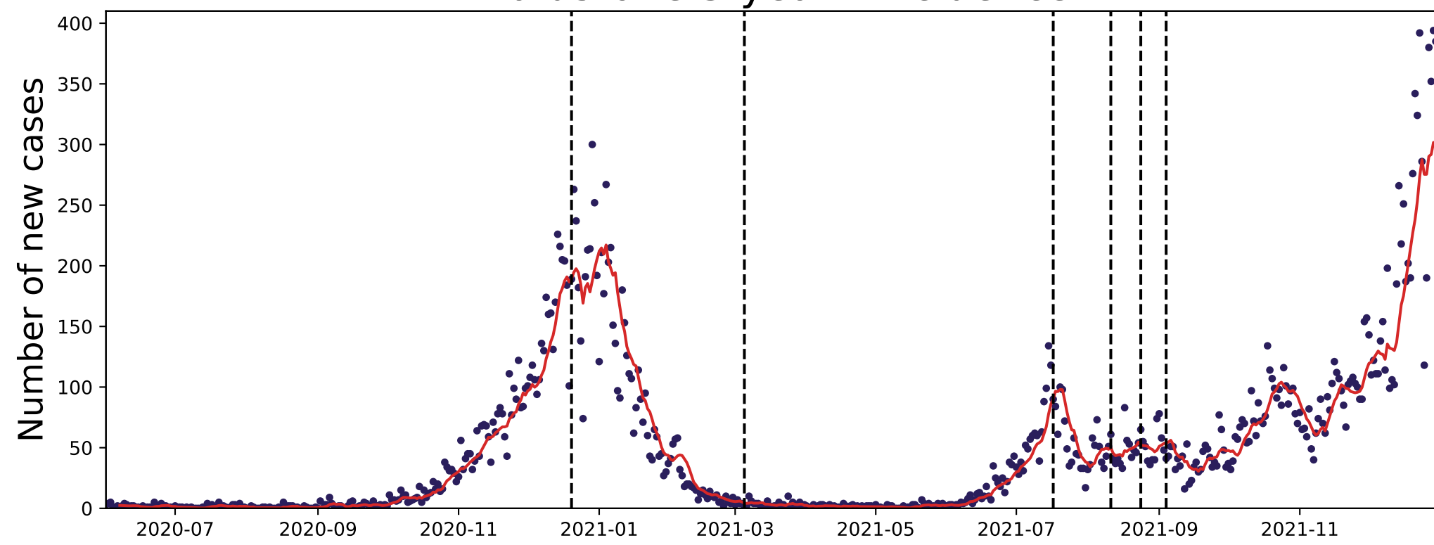
Maidstone 5-year - incidence
