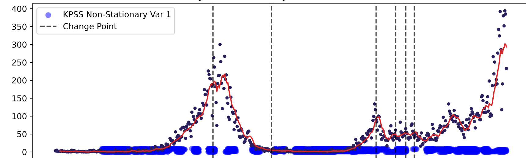
60 days - Maidstone 5-year - incidence: KPSS
