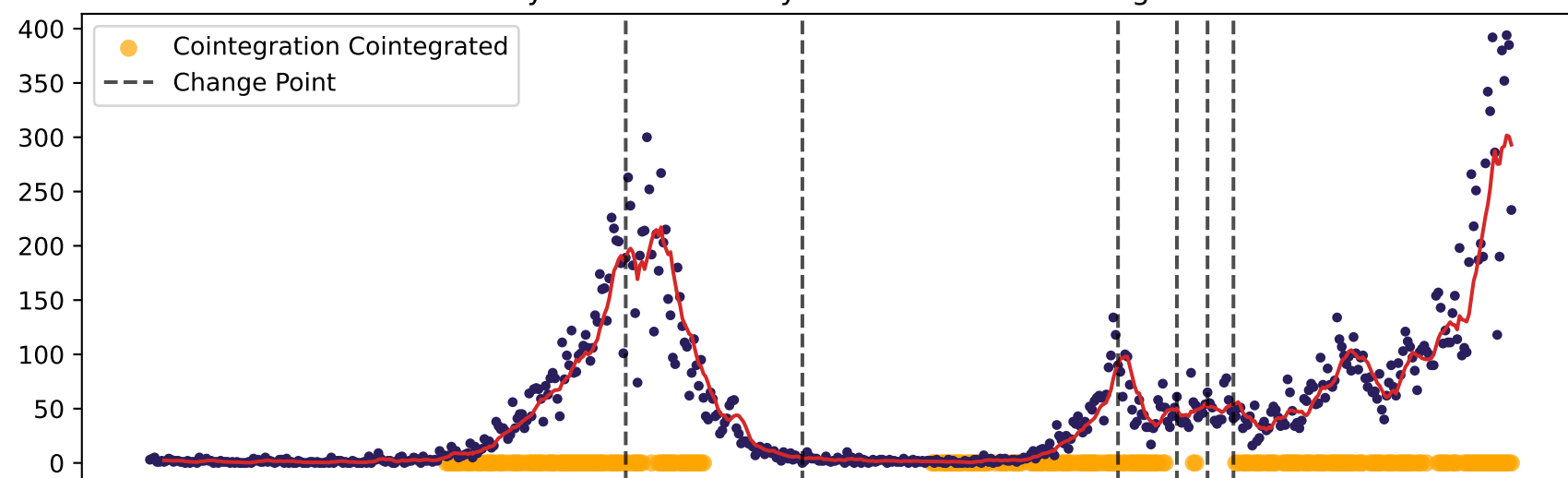
100 days - Maidstone 5-year - incidence: Cointegration
