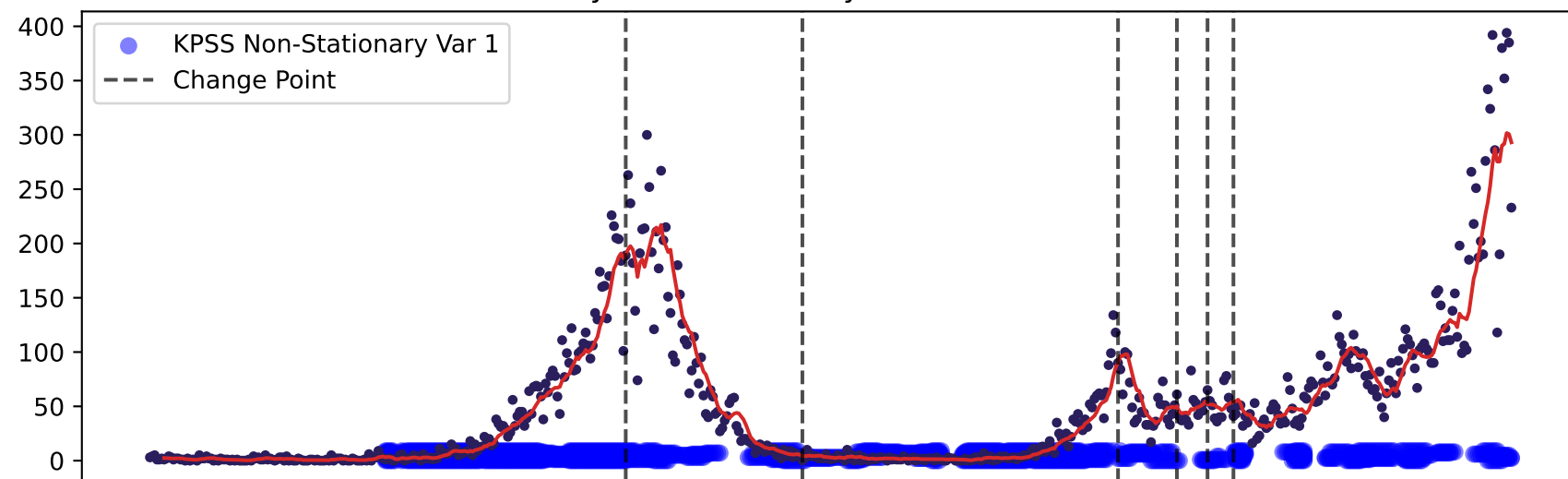
100 days - Maidstone 5-year - incidence: KPSS
