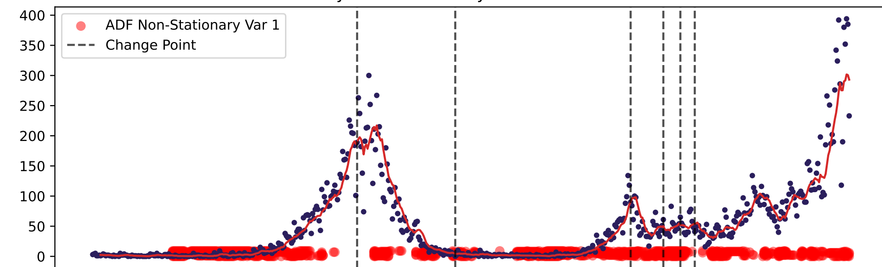
60 days - Maidstone 5-year - incidence: ADF
