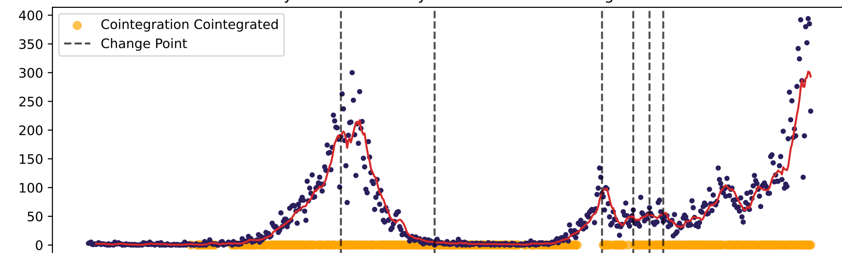
60 days - Maidstone 5-year - incidence: Cointegration
