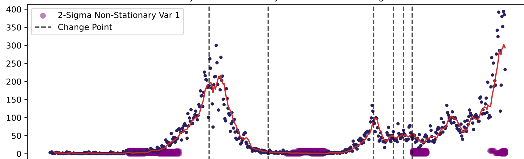
100 days - Maidstone 5-year - incidence: 2-Sigma
