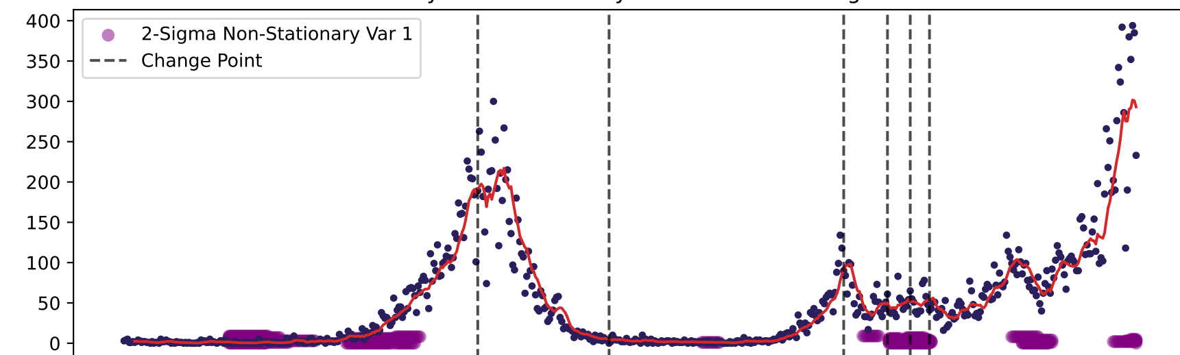
60 days - Maidstone 5-year - incidence: 2-Sigma
