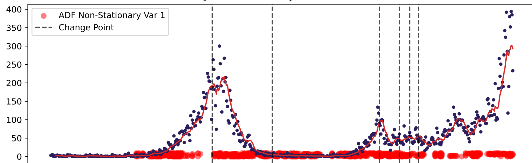
100 days - Maidstone 5-year - incidence: ADF
