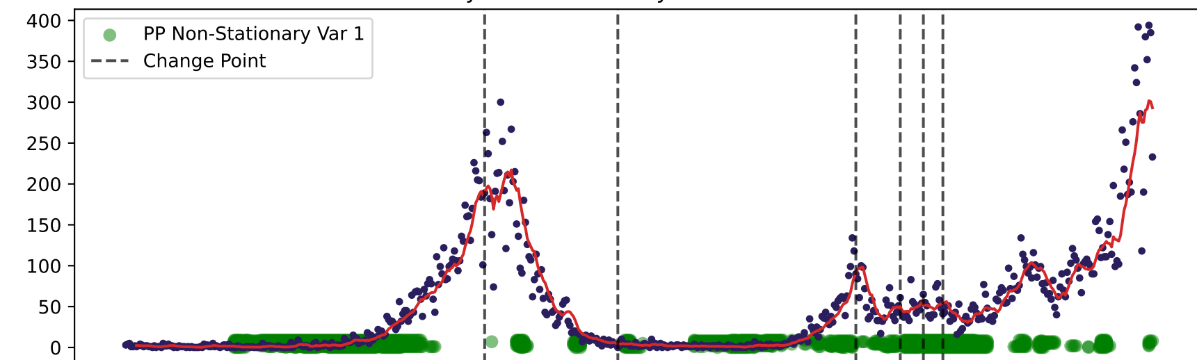
60 days - Maidstone 5-year - incidence: PP
