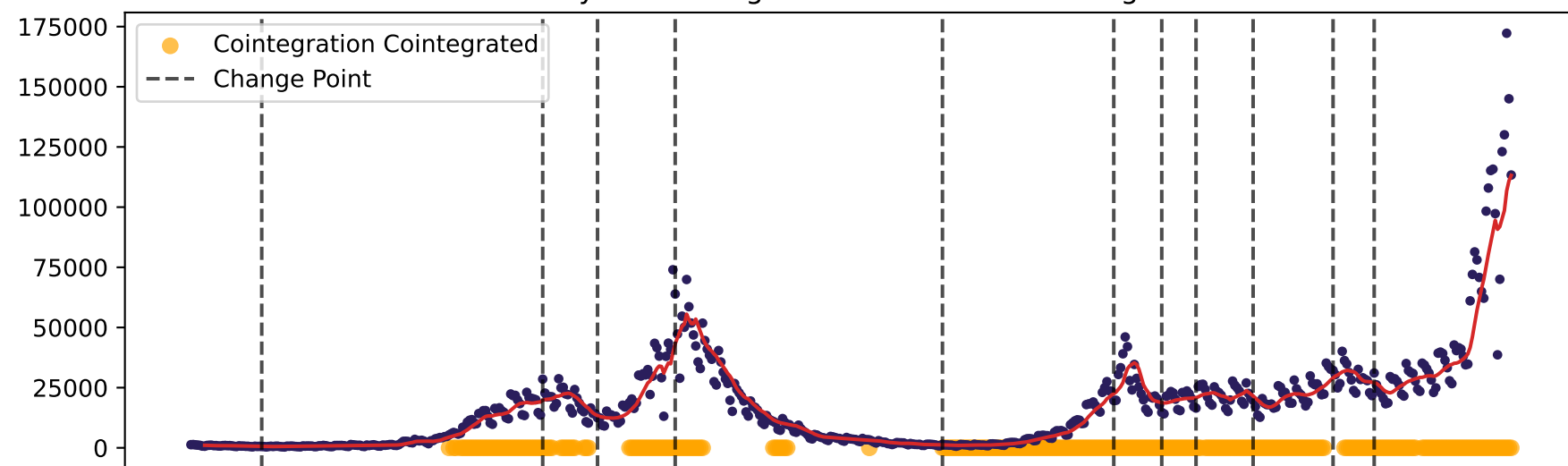
100 days - NHS Regional - detrended: Cointegration
