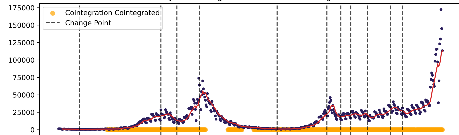
60 days - NHS Regional - detrended: Cointegration
