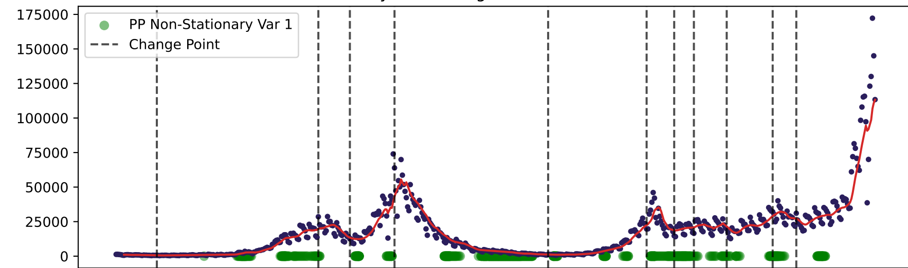
60 days - NHS Regional - detrended: PP
