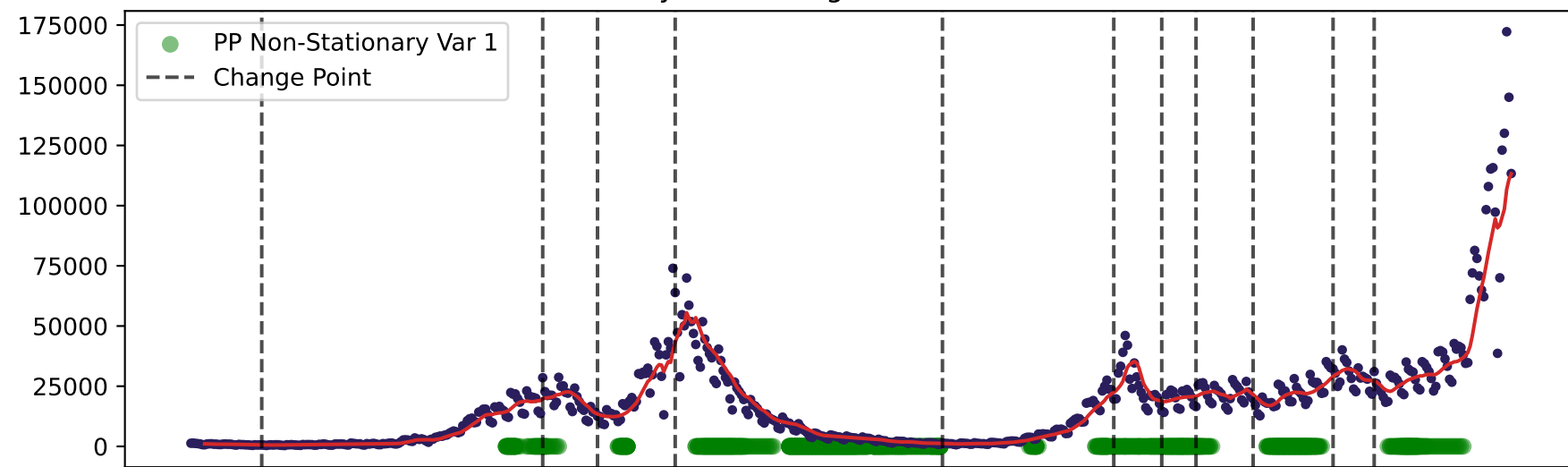
100 days - NHS Regional - detrended: PP
