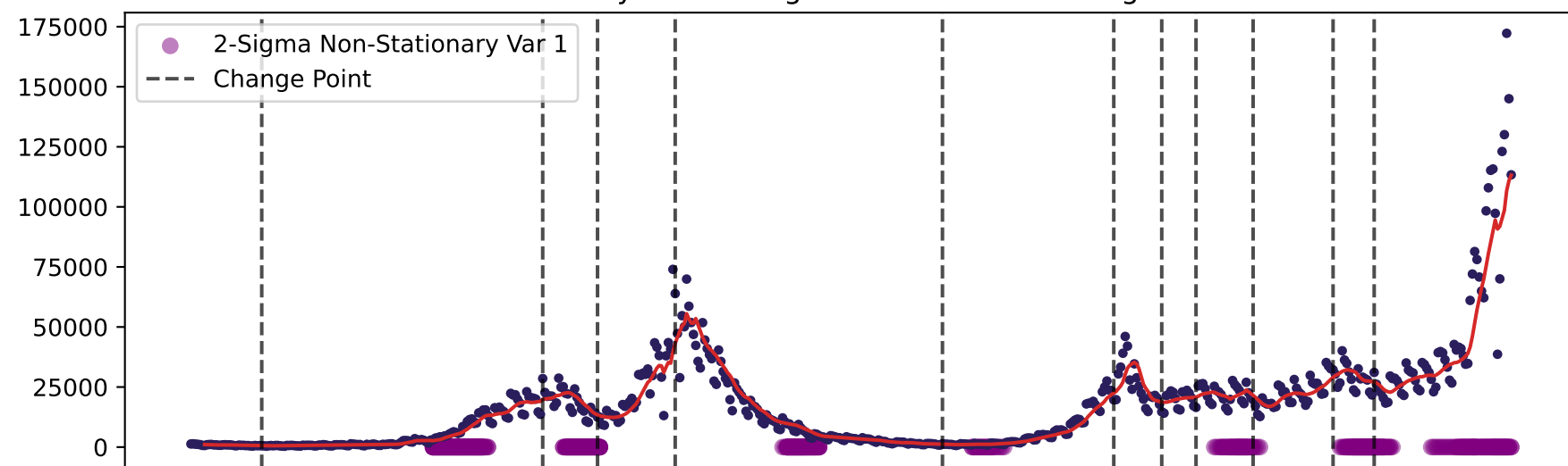
100 days - NHS Regional - detrended: 2-Sigma
