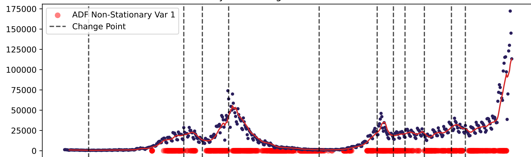
100 days - NHS Regional - detrended: ADF
