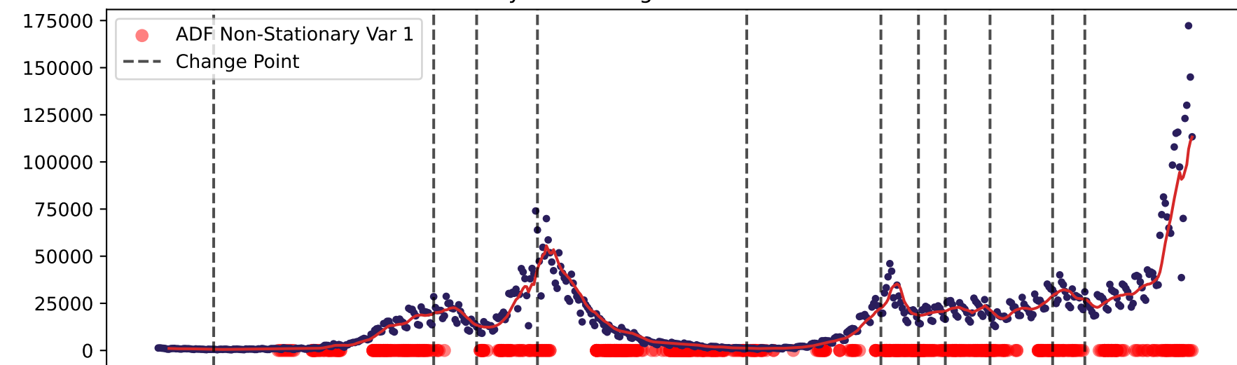
60 days - NHS Regional - detrended: ADF
