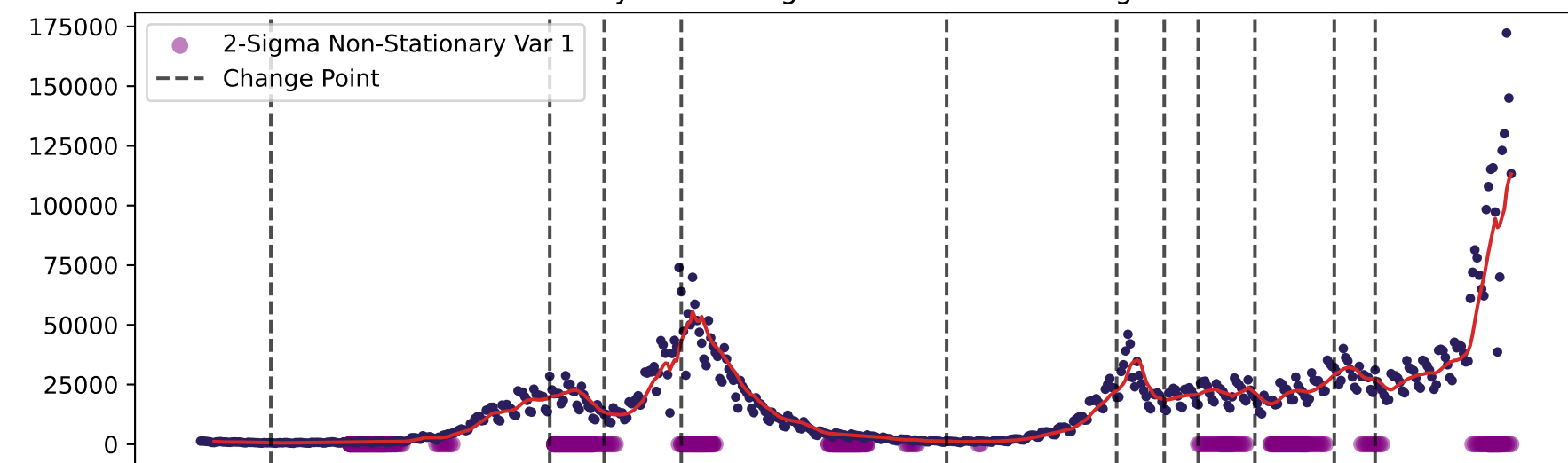
60 days - NHS Regional - detrended: 2-Sigma
