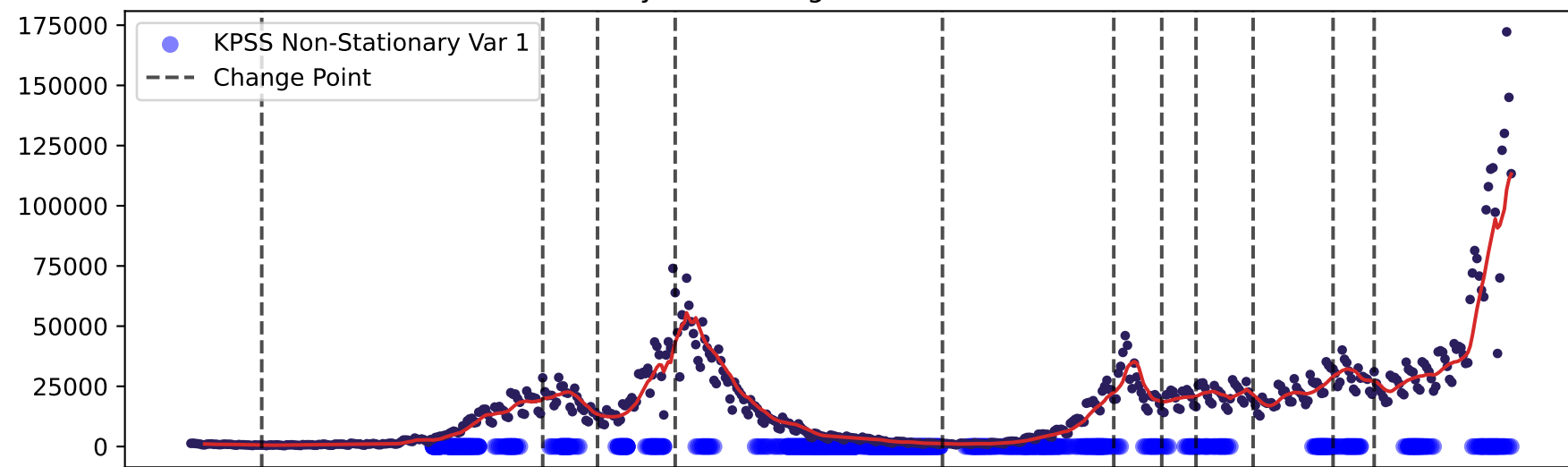
100 days - NHS Regional - detrended: KPSS
