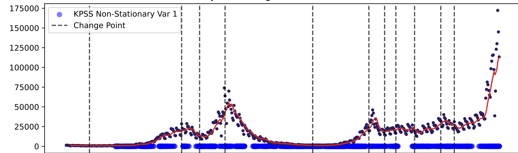
60 days - NHS Regional - detrended: KPSS
