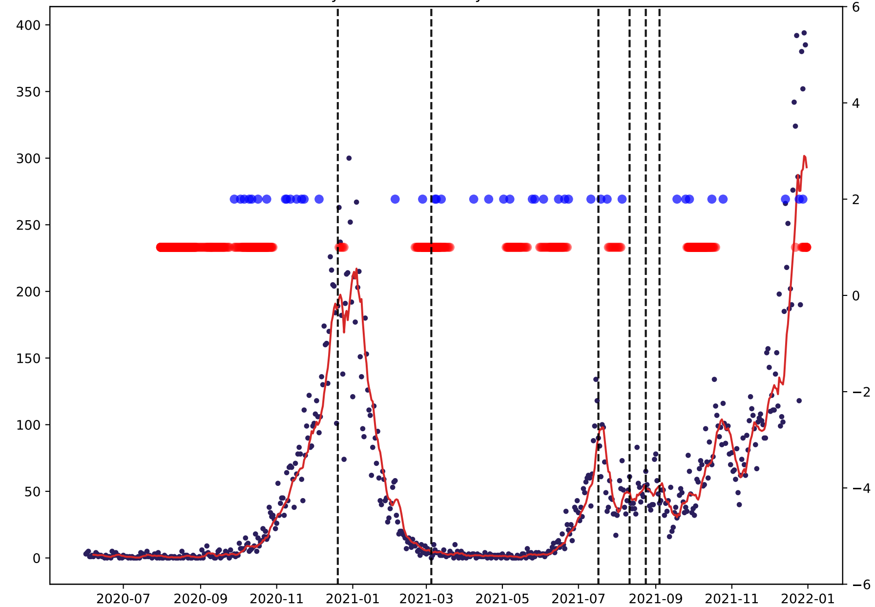
60 days - Maidstone 10-year - detrended
