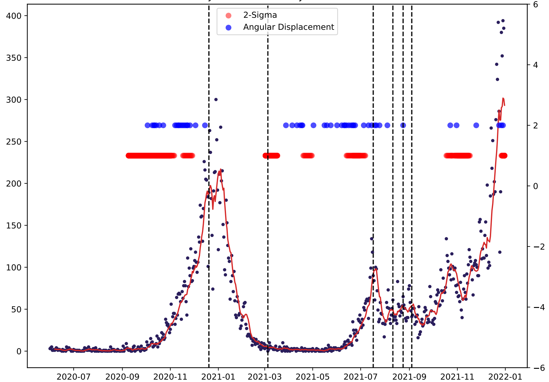
100 days - Maidstone 10-year - detrended
