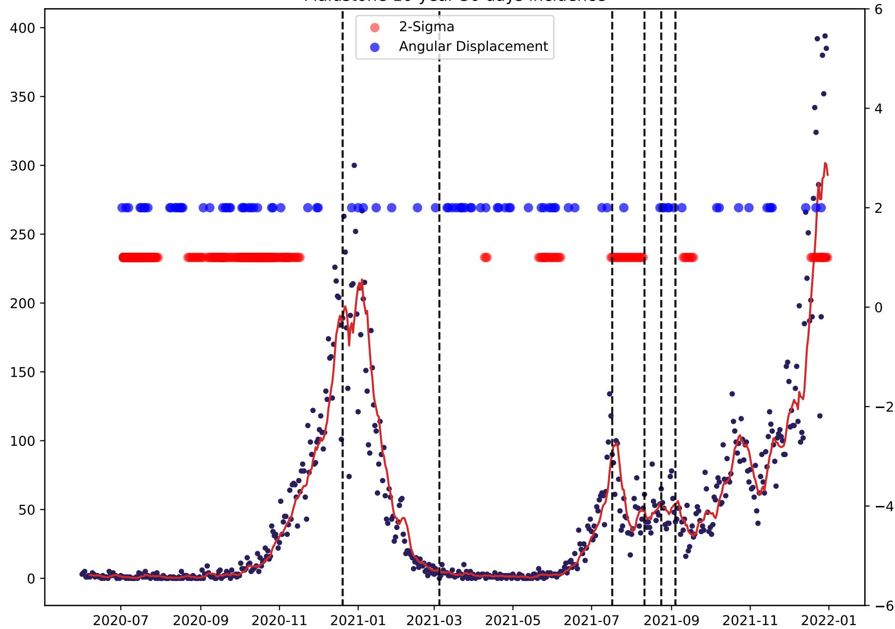
Maidstone 10-year 30 days incidence
