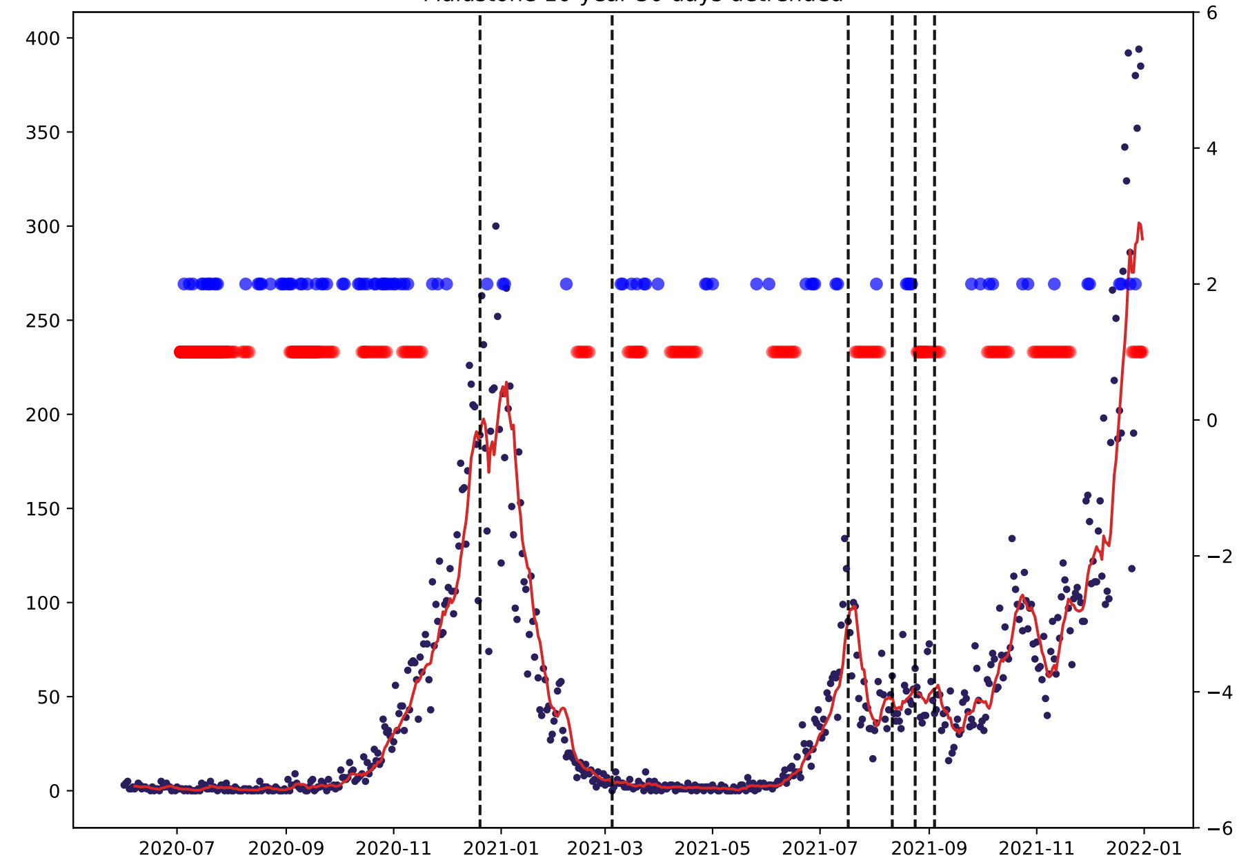
Maidstone 10-year 30 days detrended
