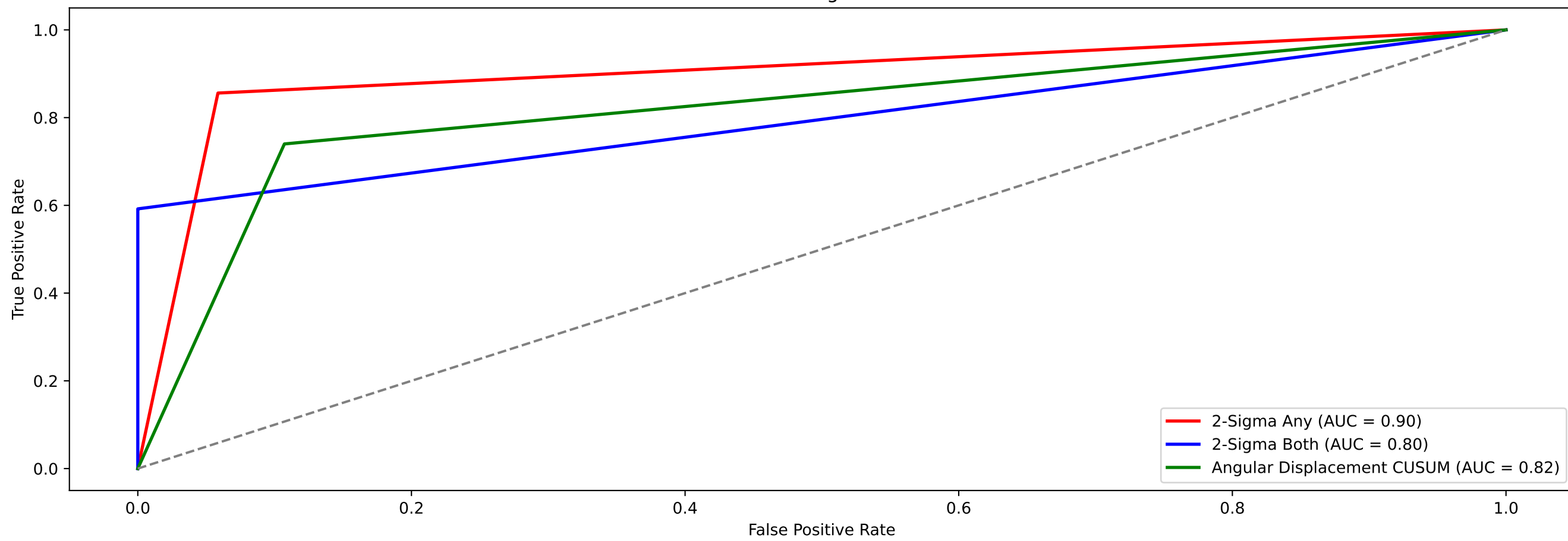
ROC Curve for Eigenvector Tests
