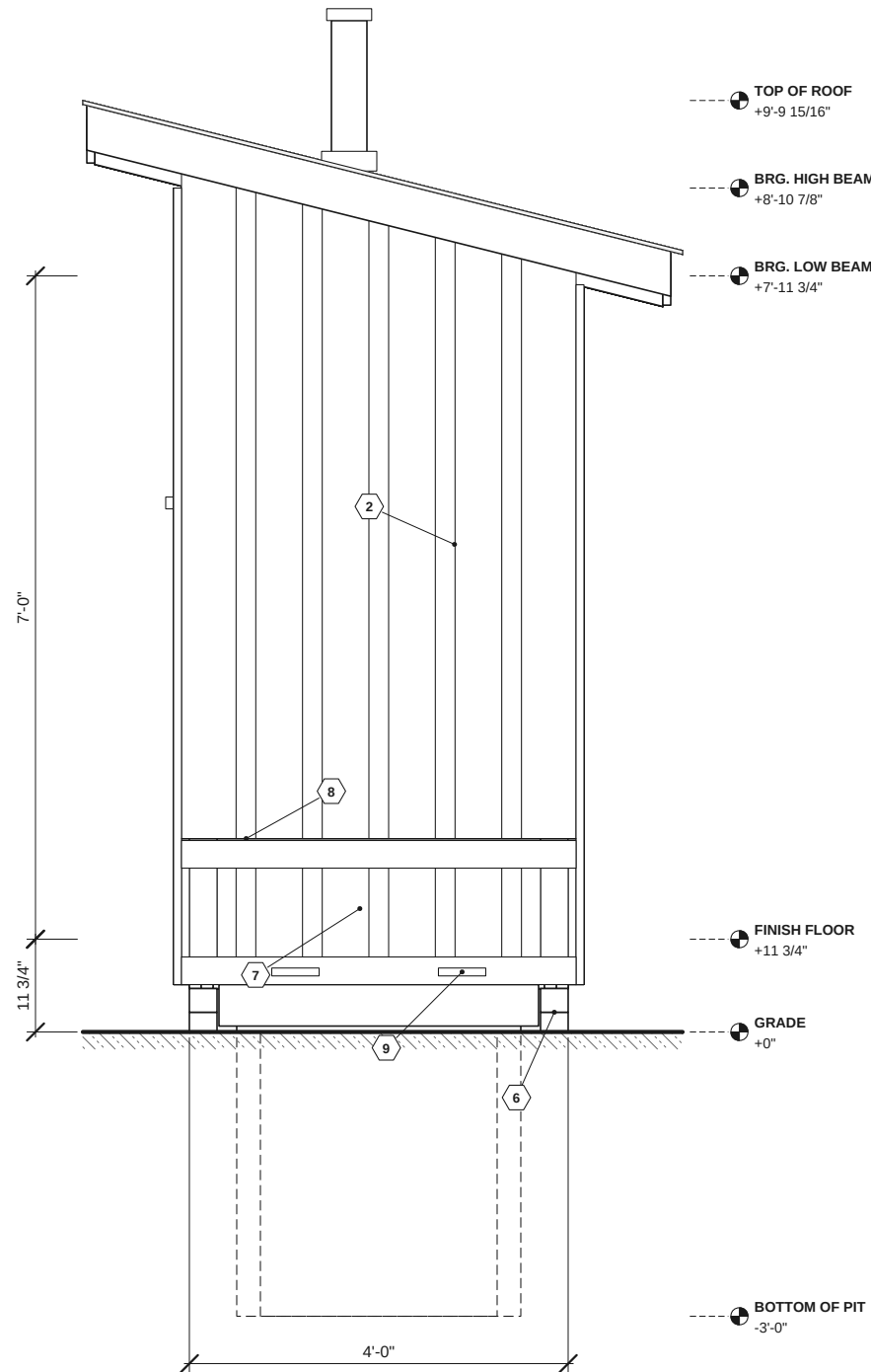
2 BACK (REMOVABLE PANEL) ELEVATION
