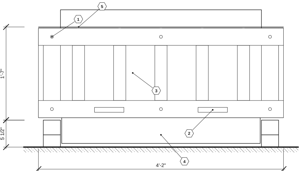
1 REMOVABLE BACK PANEL (FROM OUTSIDE) SCALE: 1" = 1'-0"
