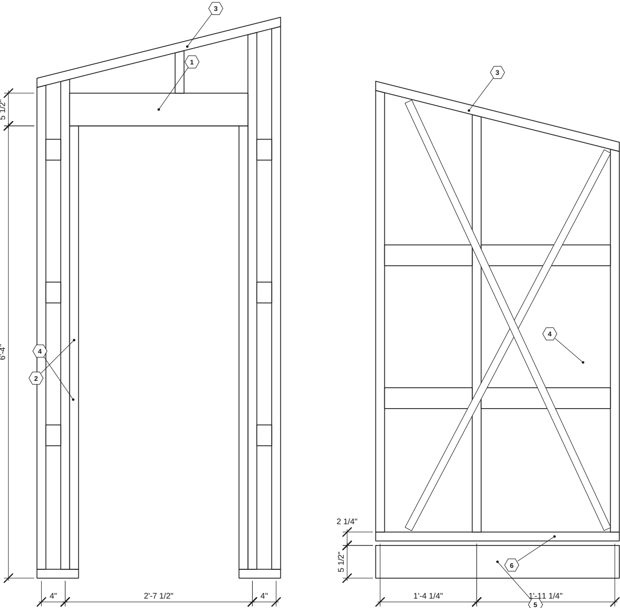
1 FRONT WALL FRAMING (FROM OUTSIDE) SCALE: 3/4" = 1'-0"
