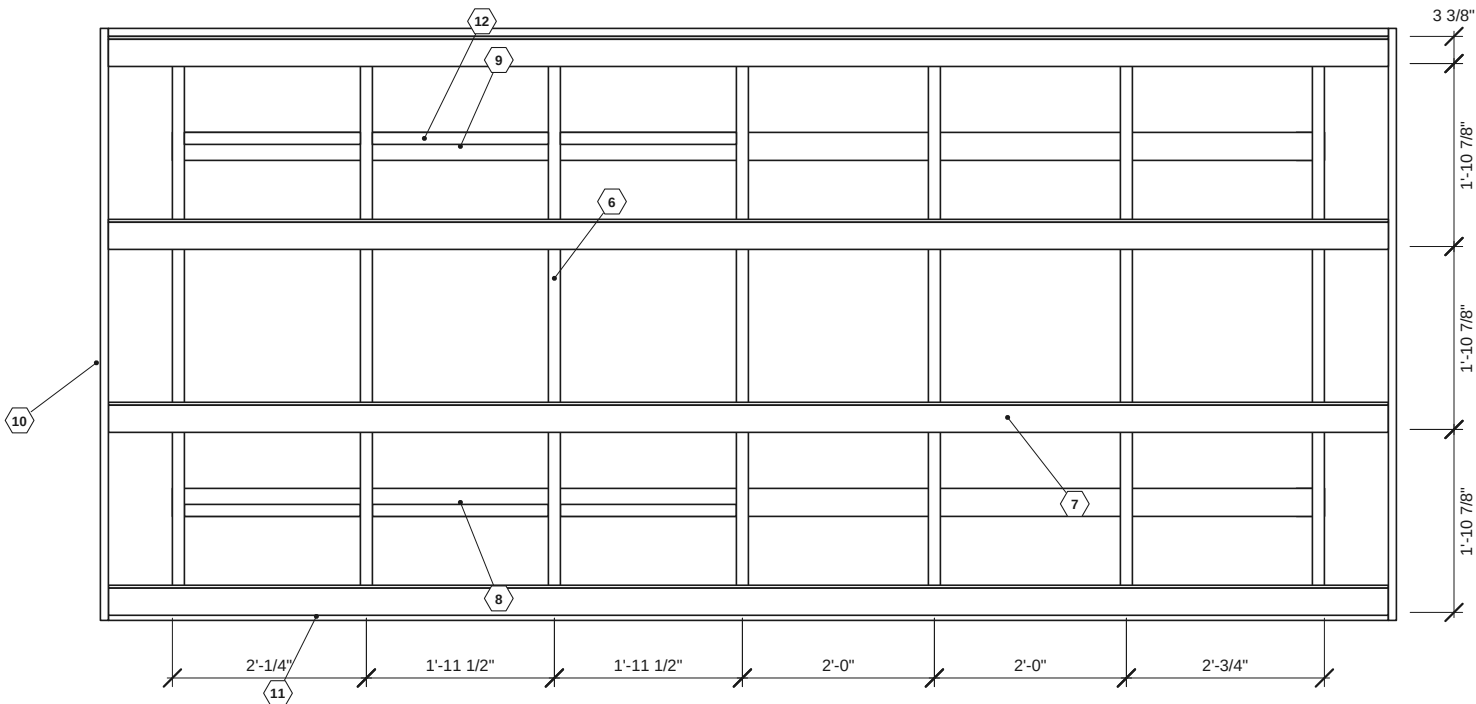
2 ROOF FRAMING PLAN
