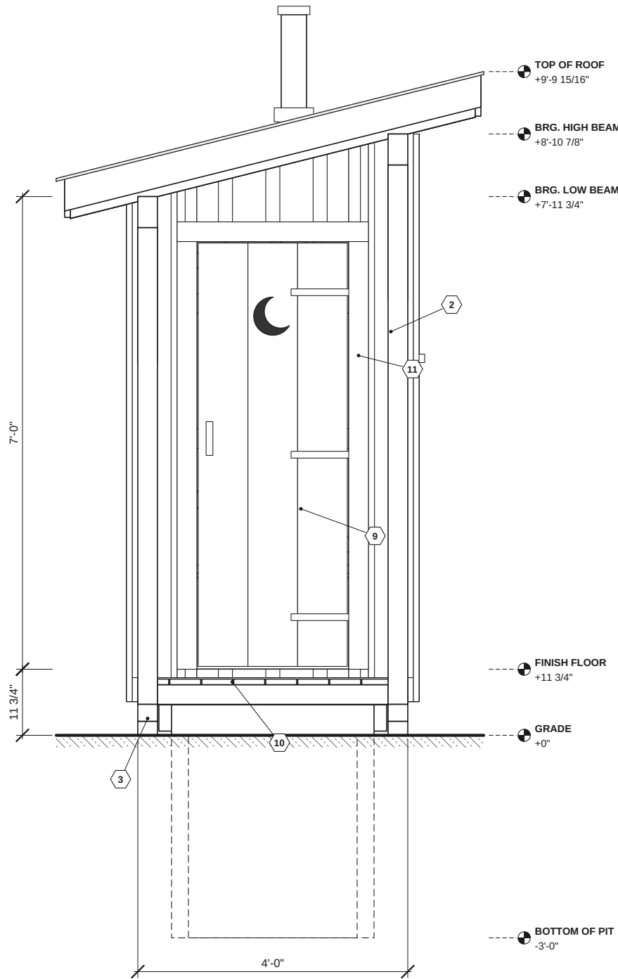
2 FRONT (DOOR / DECK) ELEVATION
