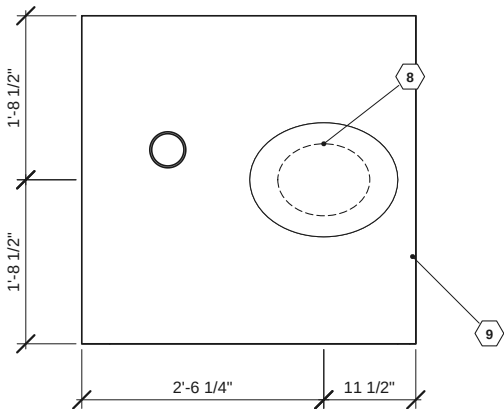
3 BENCH TOP (SEAT LID CLOSED) SCALE: 1/2" = 1'-0"
