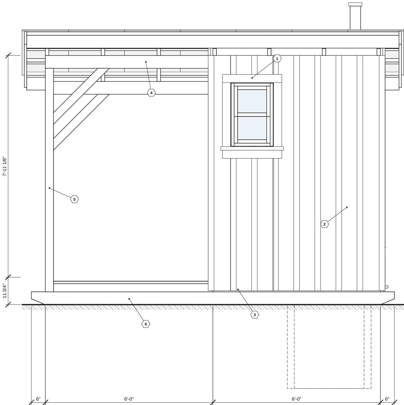
1 RIGHT (HIGH / WINDOW SIDE) ELEVATION
