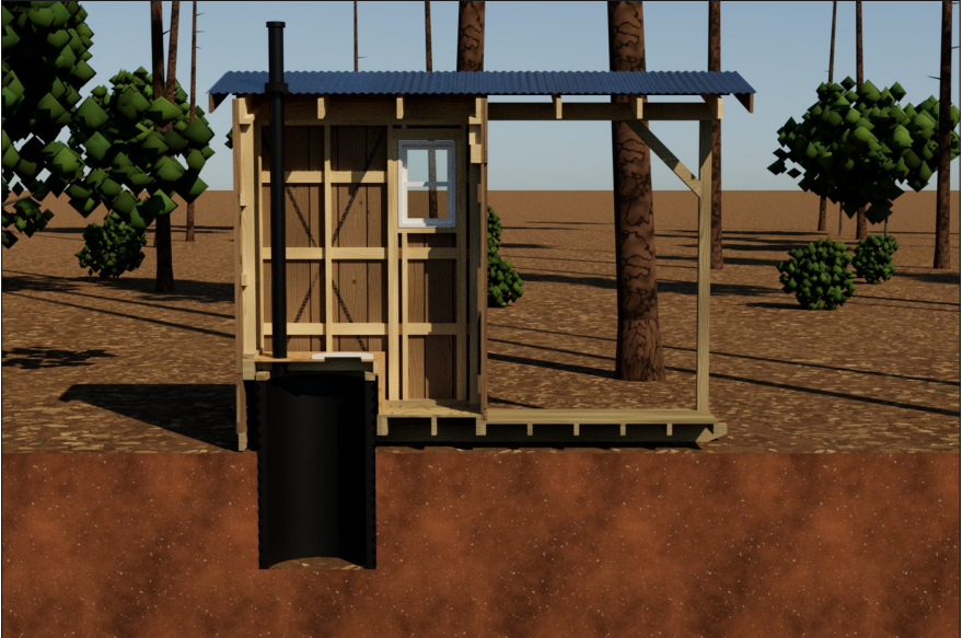
3 CUTAWAY THROUGH THE PIT CENTERLINE
