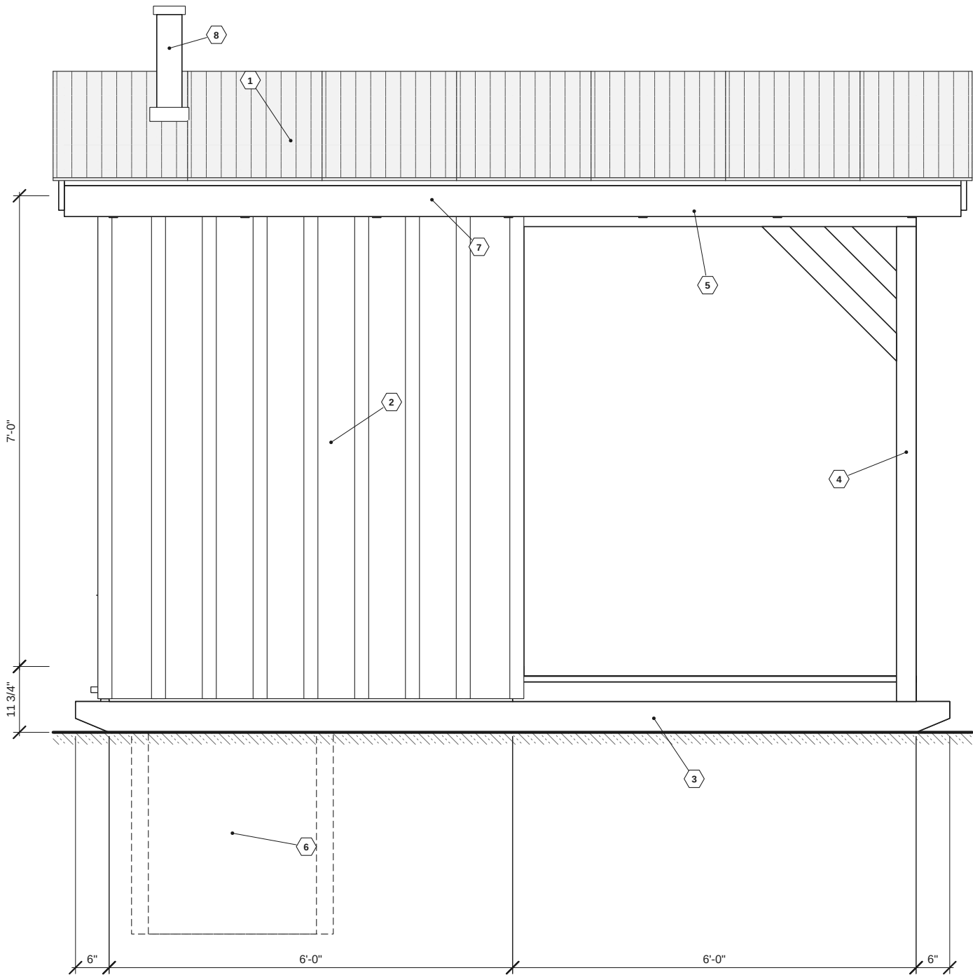
1 LEFT (LOW / EAVE SIDE) ELEVATION
