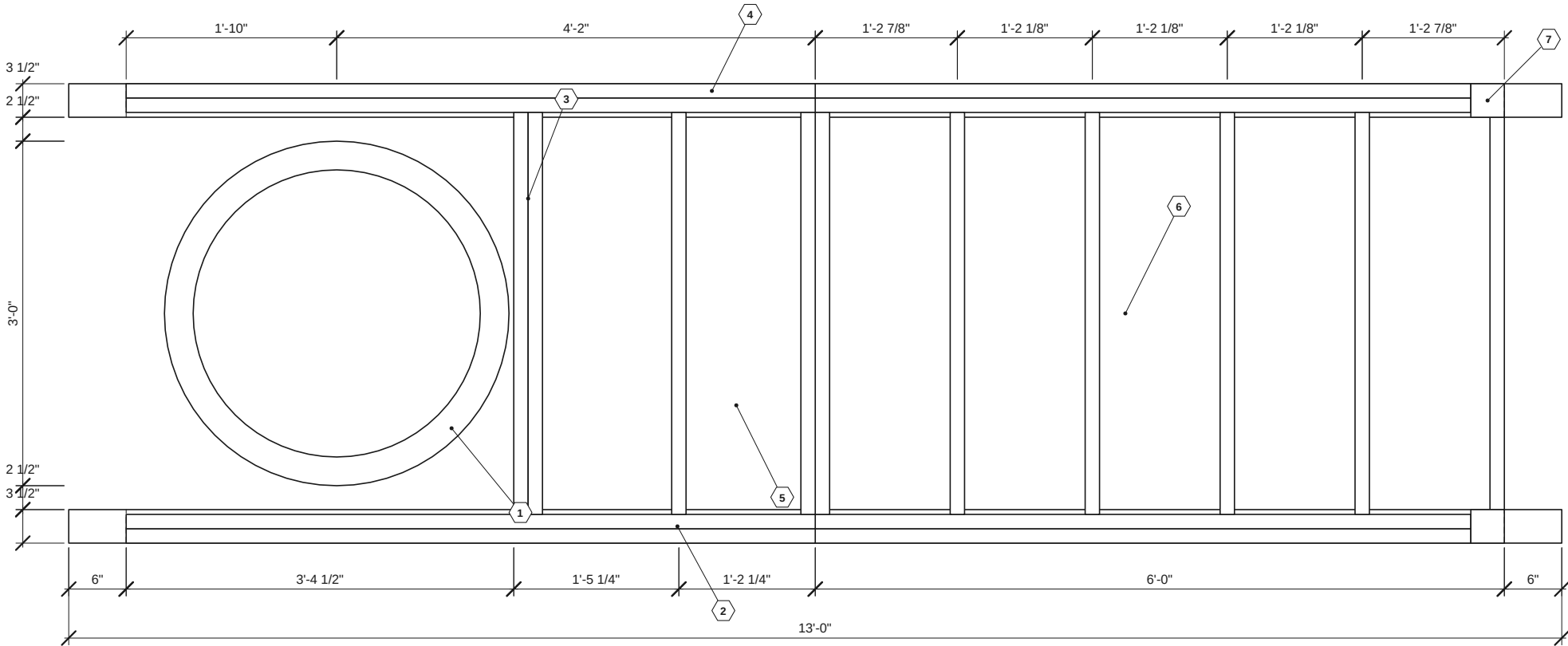
1 FOUNDATION & FLOOR FRAMING PLAN SCALE: 3/4" = 1'-0"
