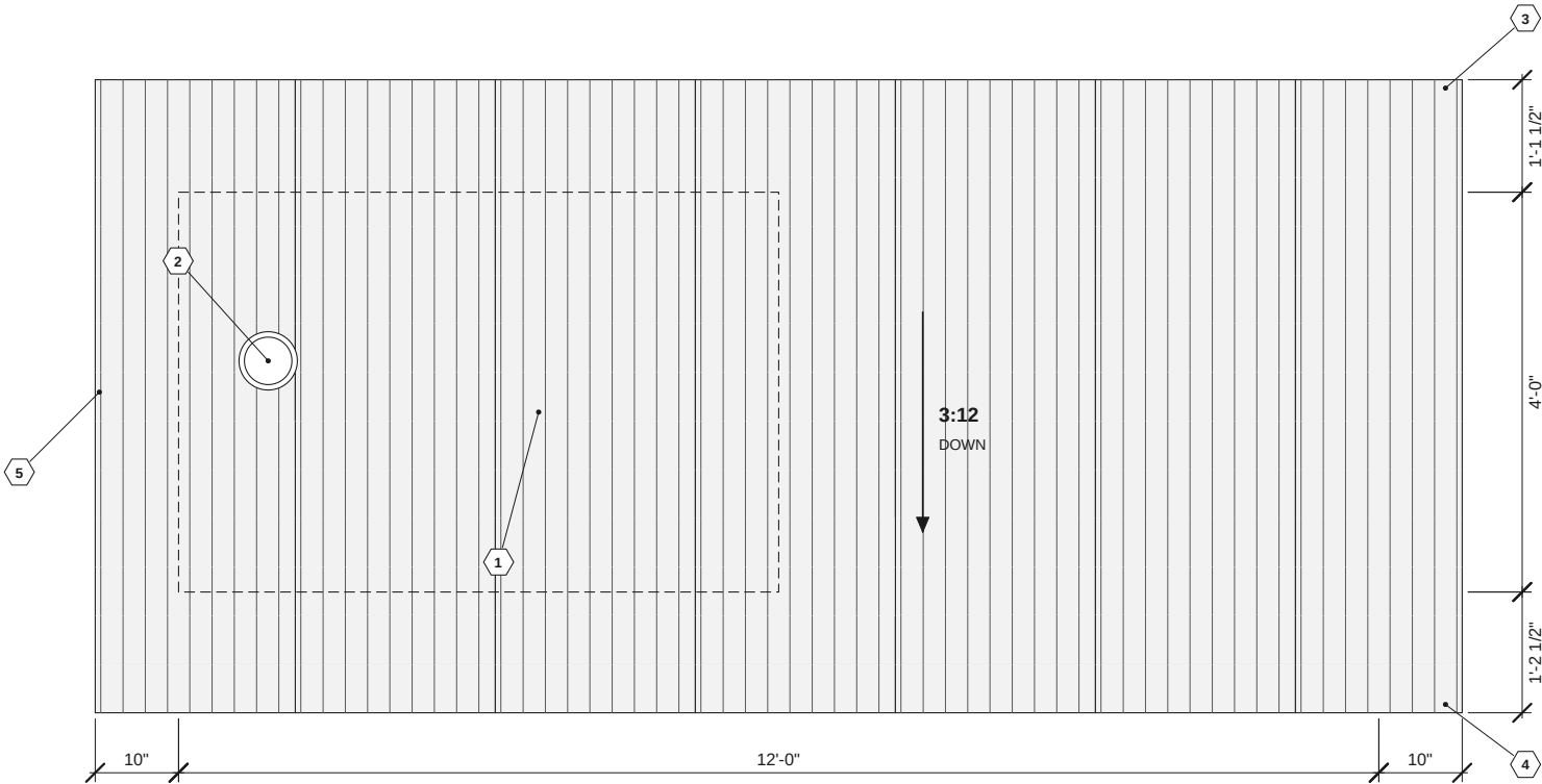
1 ROOF PLAN
