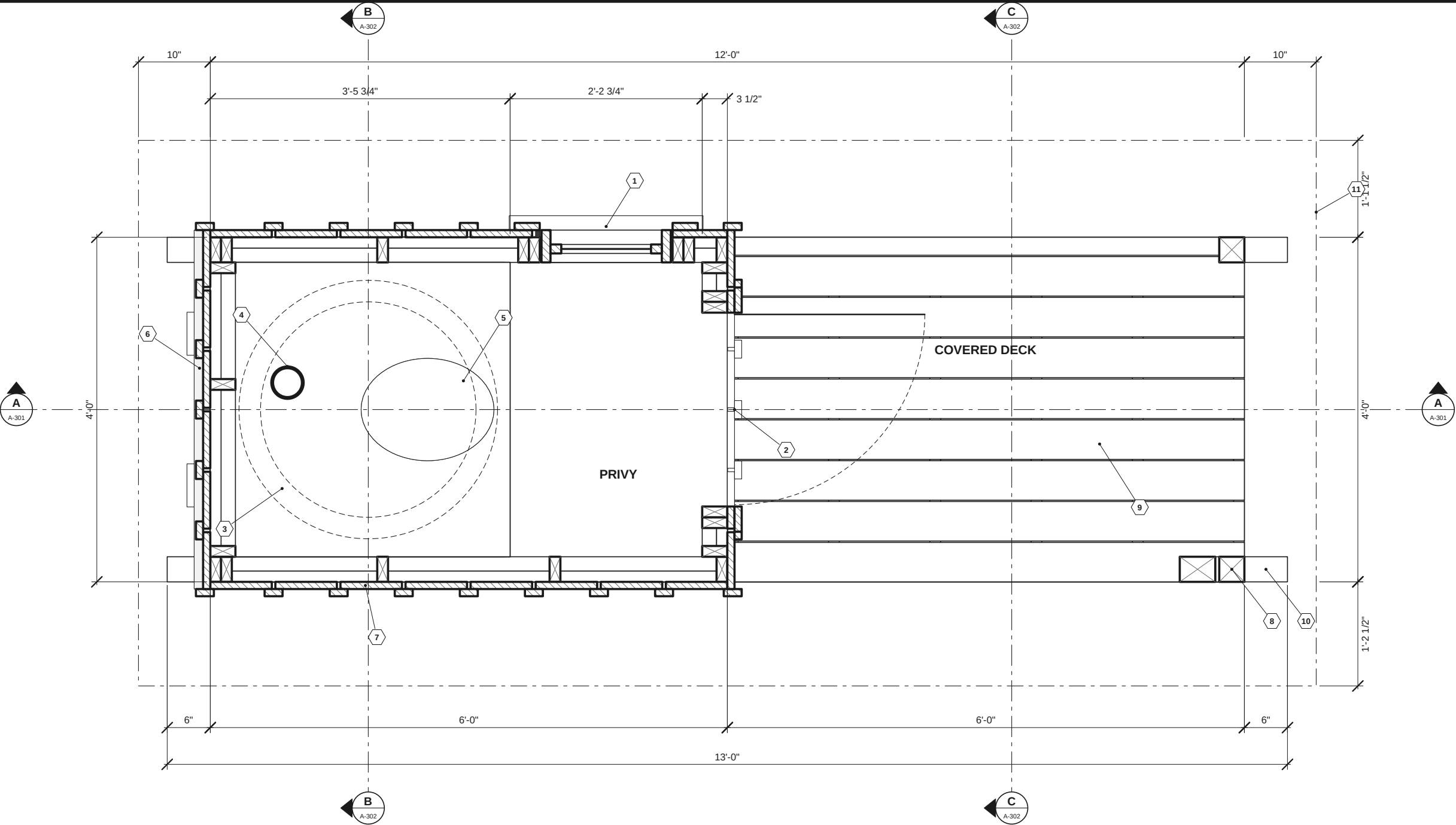
1 FLOOR PLAN SCALE: 3/4" = 1'-0"
