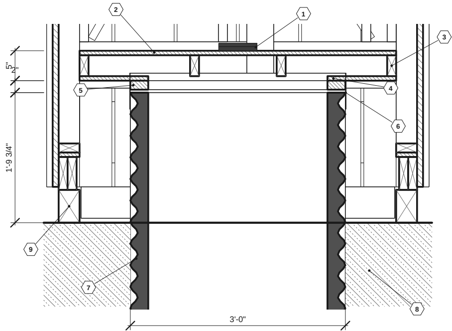
1 PIT & FLANGE DETAIL (SECTION B) SCALE: 3/4" = 1'-0"
