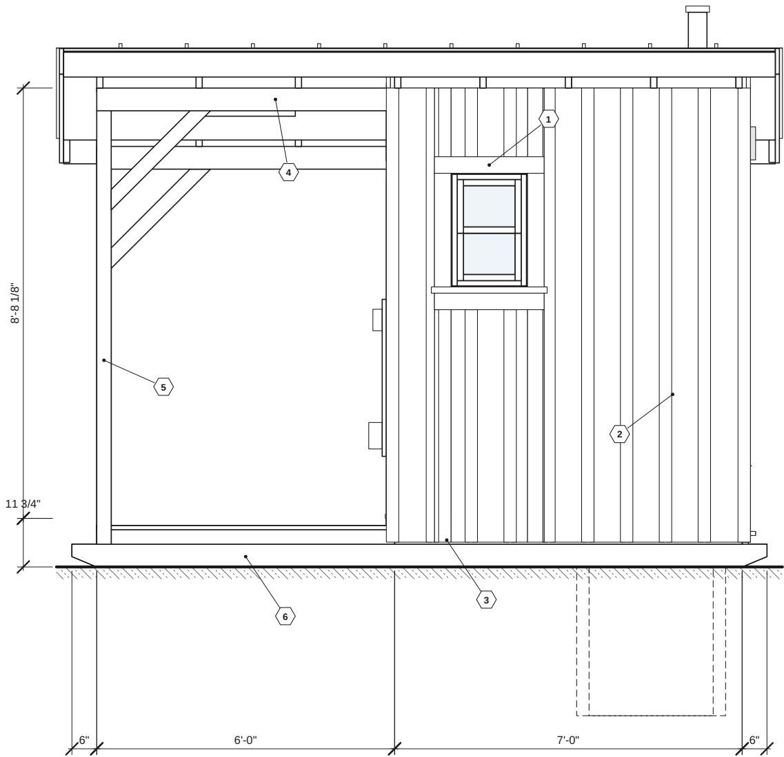
1 RIGHT (HIGH / WINDOW SIDE) ELEVATION
