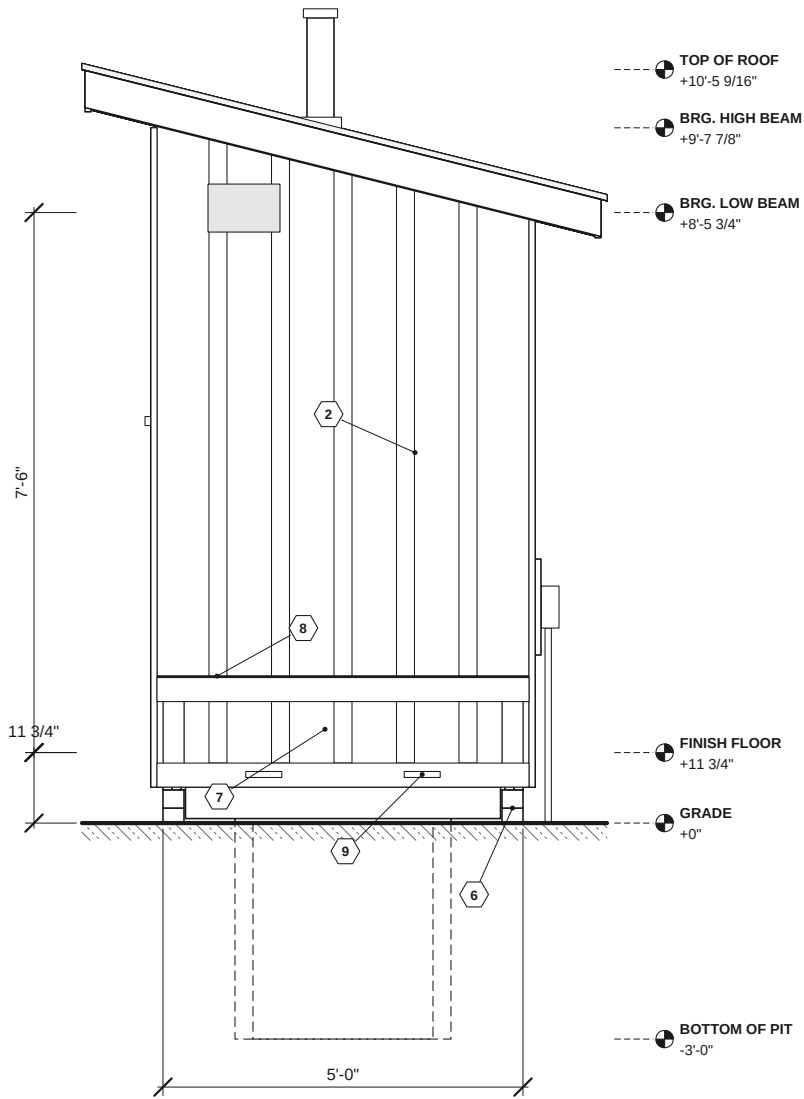
2 BACK (REMOVABLE PANEL) ELEVATION
