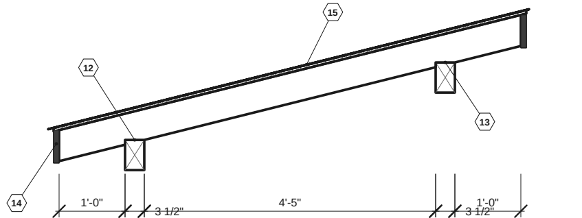
3 RAFTER LAYOUT (TYPICAL) - 7'-2 9/16" 2X6 SCALE: 1/2" = 1'-0"
