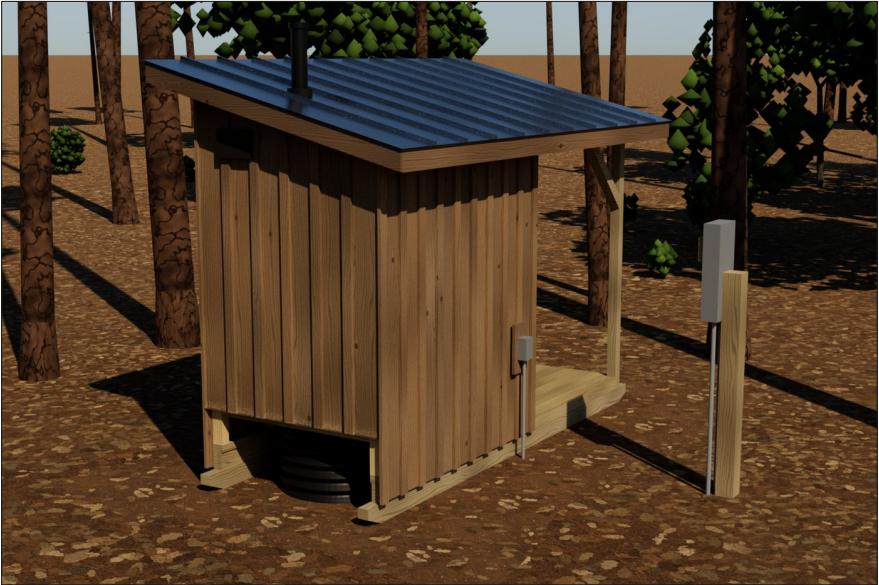
2 BACK WITH THE REMOVABLE PANEL OFF: PIPE, FLANGE AND BENCH CAVITY (MORNING SUN)
