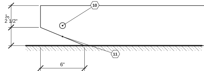
2 SKID END (BOTH ENDS) SCALE: 1-1/2" = 1'-0"
