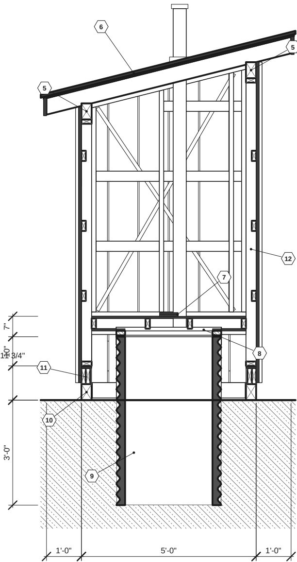
1 SECTION B: TRANSVERSE THROUGH PIT SCALE: 3/8" = 1'-0"
