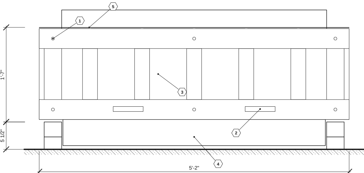
1 REMOVABLE BACK PANEL (FROM OUTSIDE) SCALE: 1" = 1'-0"
