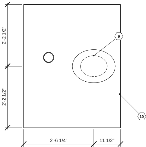
3 BENCH TOP (SEAT LID CLOSED) SCALE: 1/2" = 1'-0"
