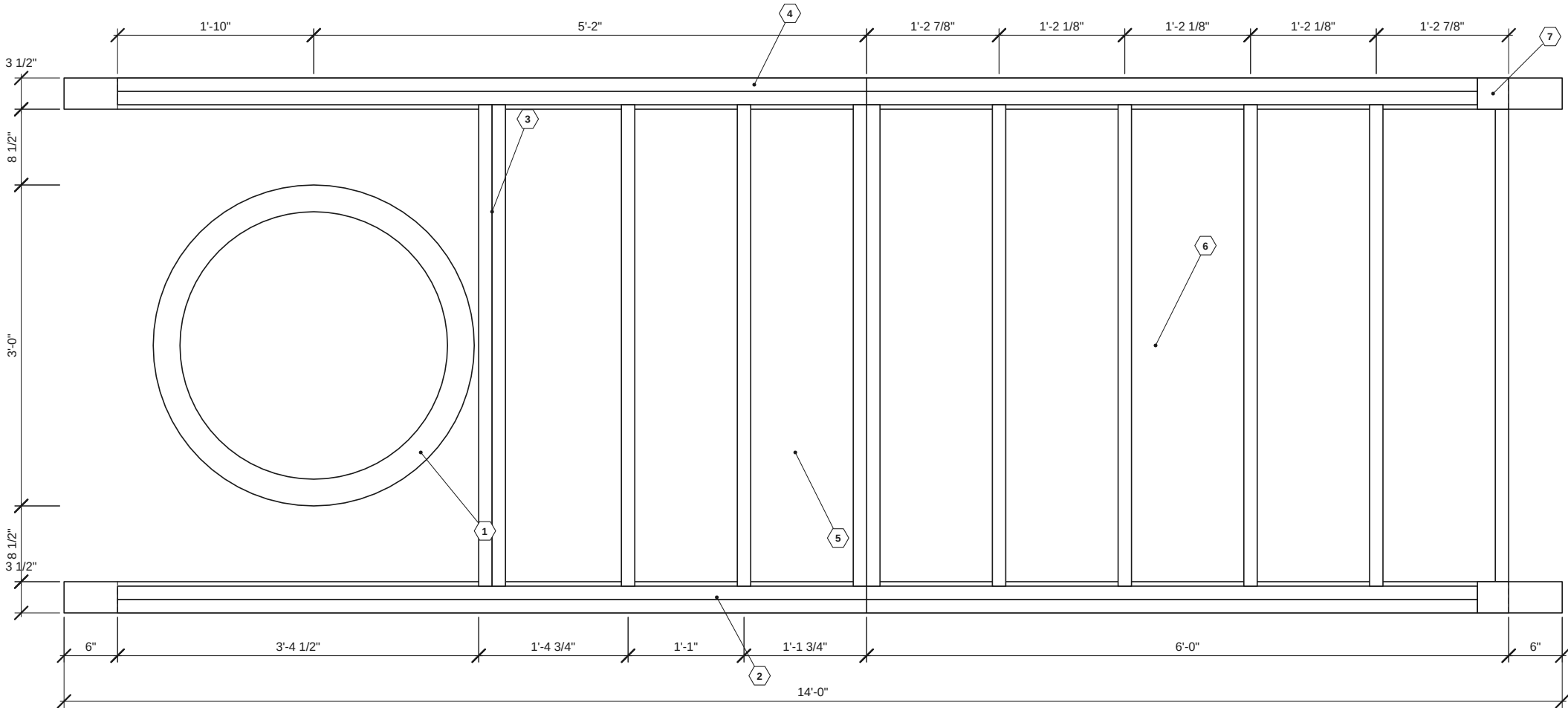
1 FOUNDATION & FLOOR FRAMING PLAN SCALE: 3/4" = 1'-0"
