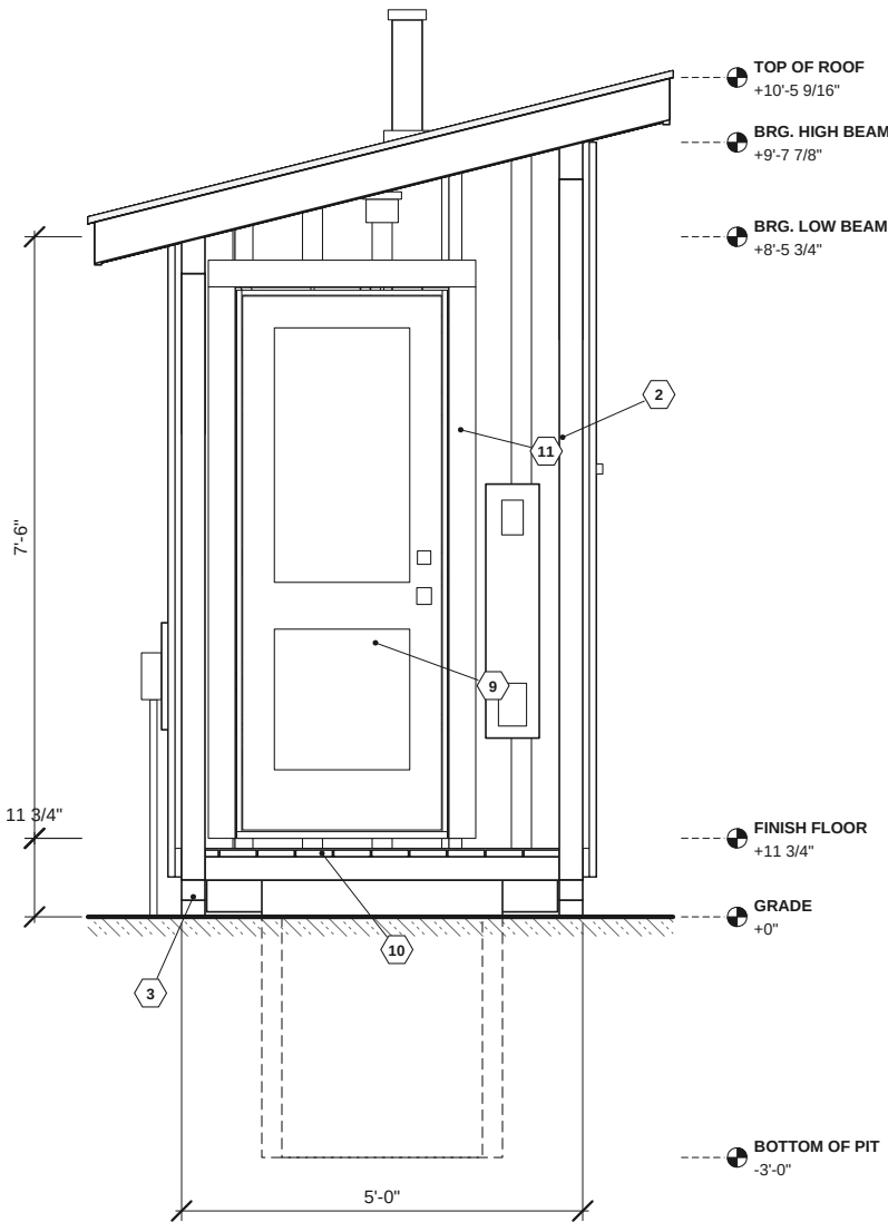
2 FRONT (DOOR / DECK) ELEVATION
