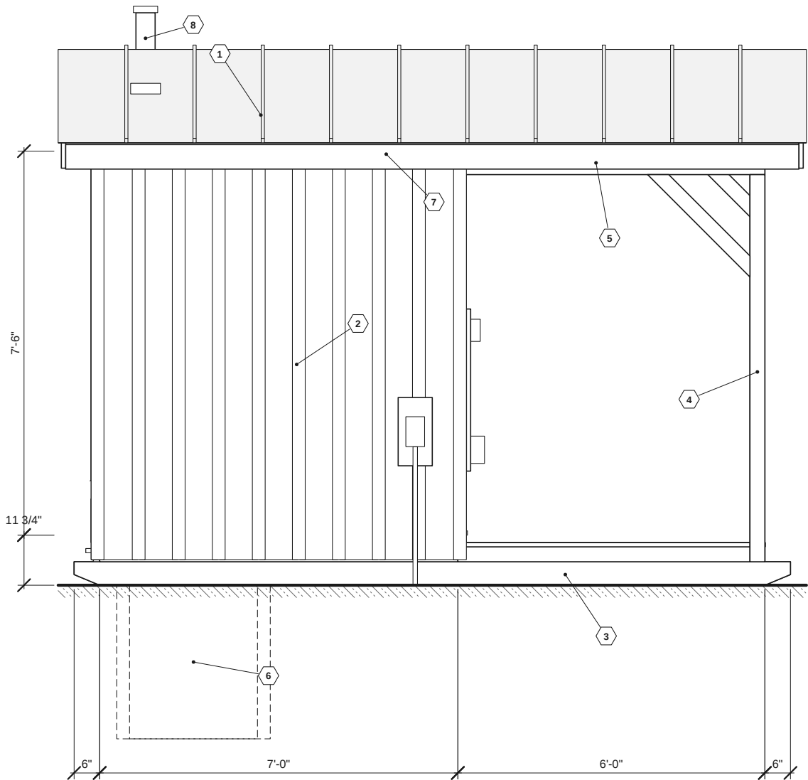
1 LEFT (LOW / EAVE SIDE) ELEVATION
