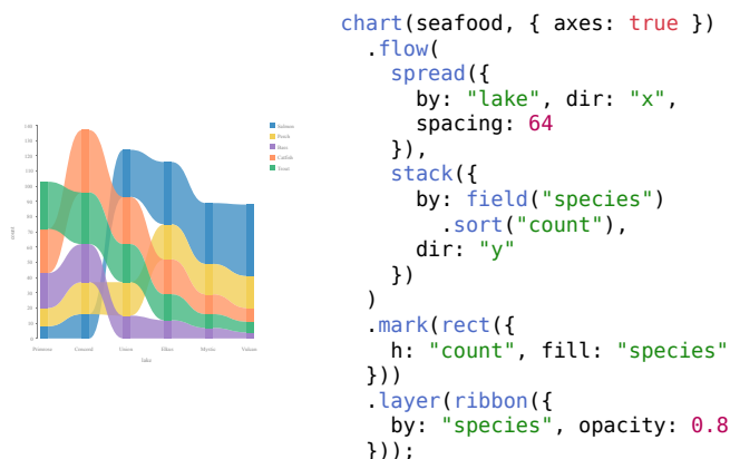
Figure 2: A GoFish ribbon chart: operators arrange the rectangles, and a relational mark connects them.
