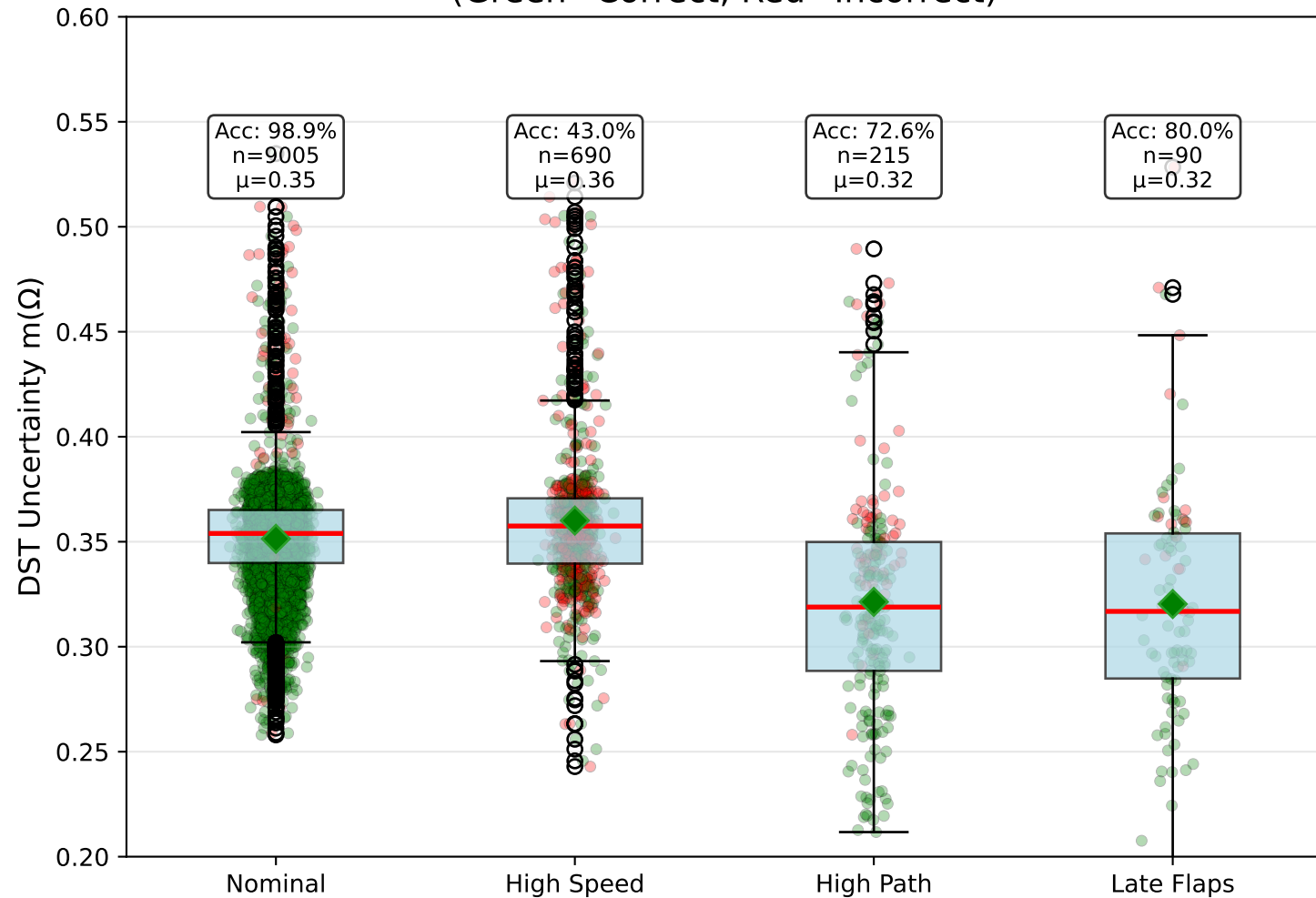
Uncertainty Distribution by True Class (Green=Correct, Red=Incorrect)
