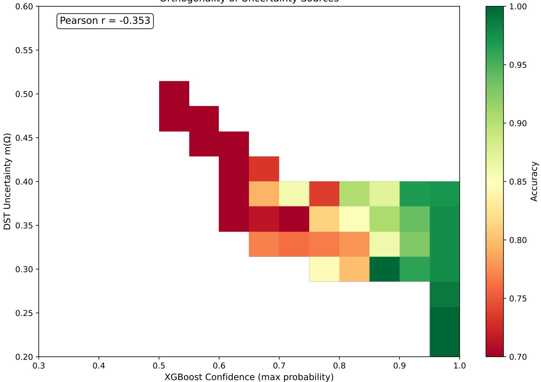
Orthogonality of Uncertainty Sources
