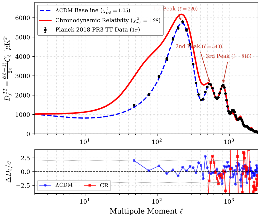
Planck 2018 PR3 CMB Temperature Power Spectrum
