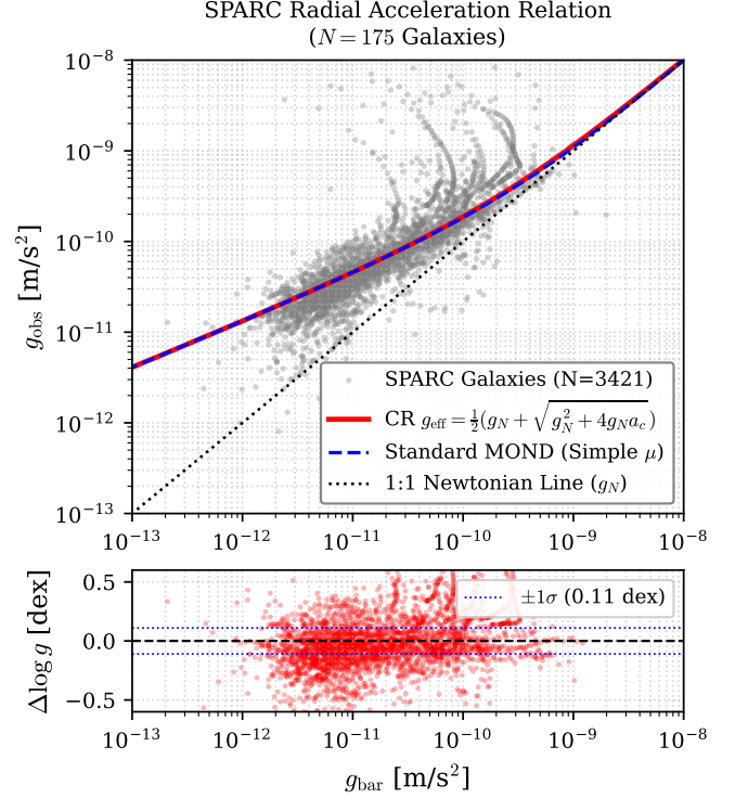
FIG. 2. The Radial Acceleration Relation (RAR) across 175 SPARC galaxies. The solid line represents the algebraic root prediction g_{\text{eff}}(g_N) , matching empirical data across five decades in acceleration without dark matter halos.
