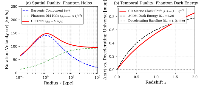
FIG. 1. The CDM Inverse-Poisson Duality. In Chronodynamic Relativity, the single scalar field \rho_s(\vec{x}, t) resolves dark sector phenomenology via dual projections: a spatial inverse-Poisson projection generating effective galactic dark matter halos, and a temporal inverse-Poisson projection generating apparent dark energy cosmic acceleration.
