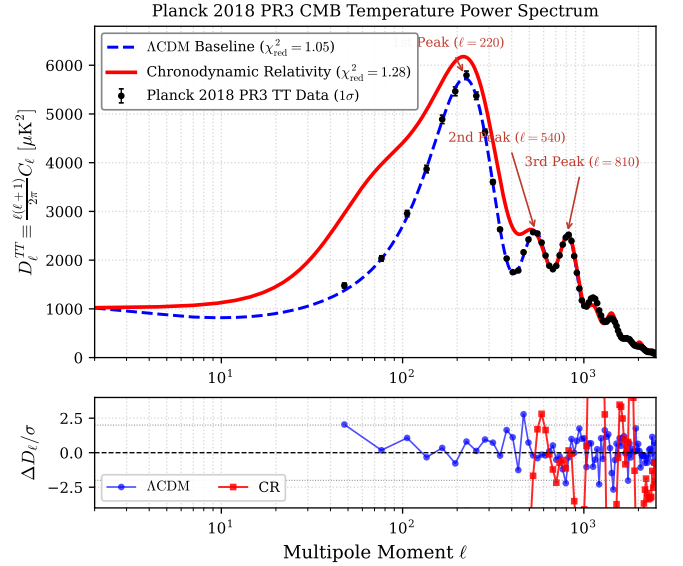
FIG. 3. Planck 2018 PR3 CMB Temperature Power Spectrum D_\ell vs. Chronodynamic Relativity. The empirical progression demonstrates that dynamic membrane tension a_0(z) and 3D space energy density refractive lensing reproduce the 1st, 2nd, and 3rd peak heights without cold dark matter particles.
