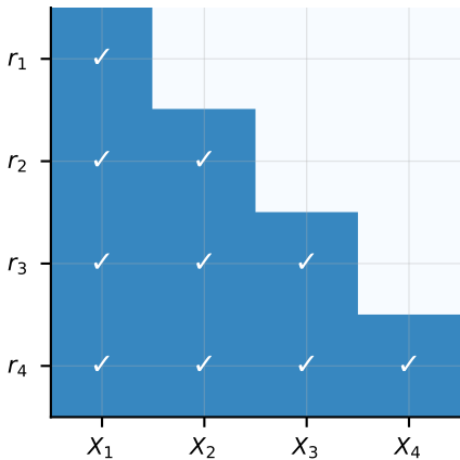
X -dependence: r_k(X_{1:k})
