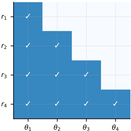
\theta -dependence: r_k(\theta_{1:k})
