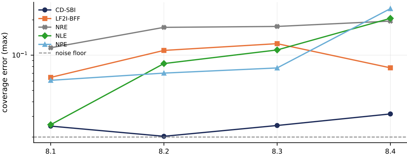
Worst-case coverage error by method
