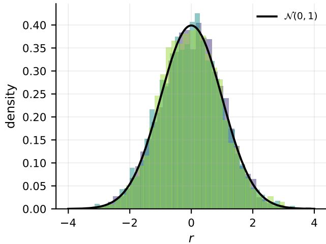
Pivot r^*(\theta_0; X) = \theta_0 - X
