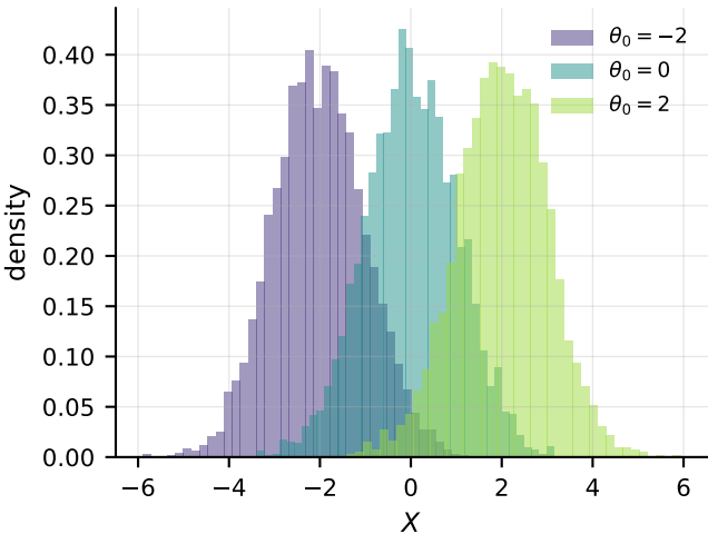
Data X \mid \theta_0
