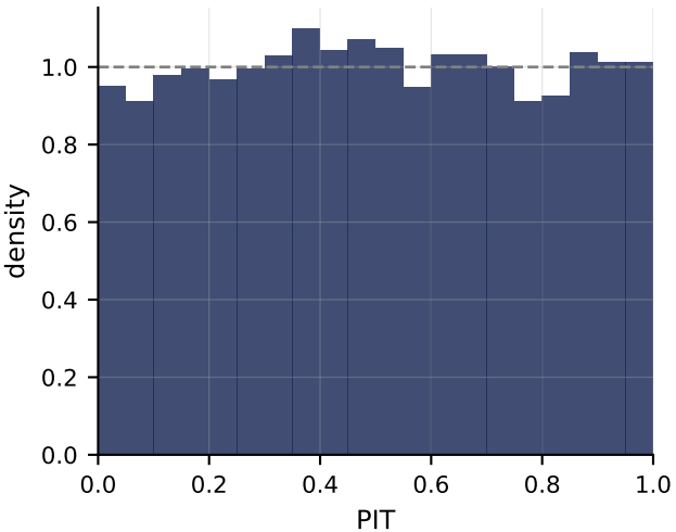
Joint Mahalanobis PIT
