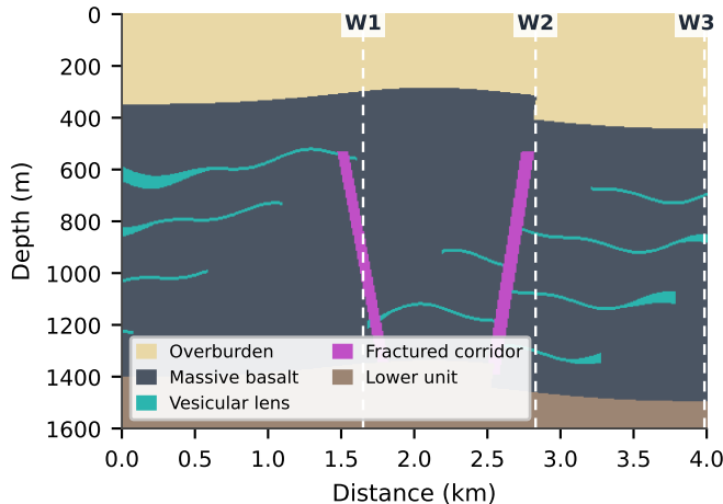
(a) Facies
