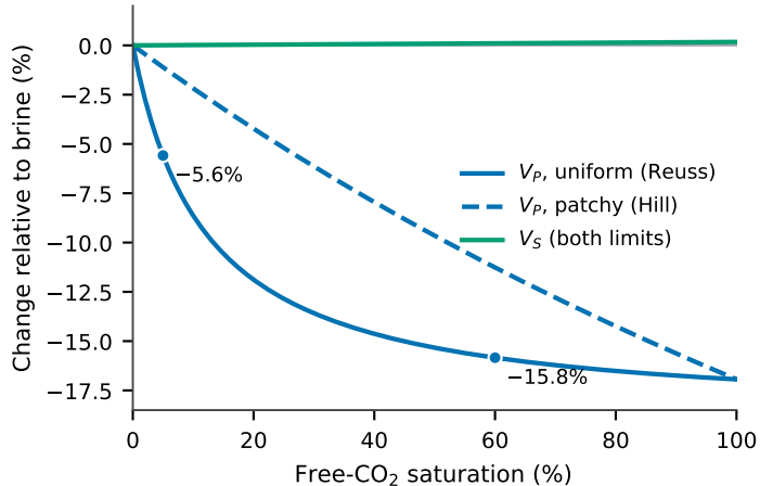
(a) Fluid substitution (no cement)
