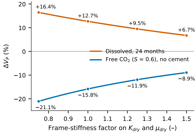
(b) Sensitivity to frame stiffness
