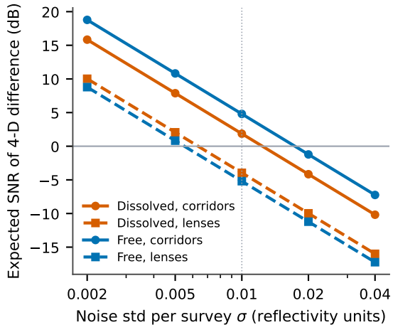
(a) Detectability vs noise
