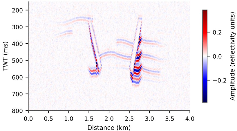
(b) Free CO 2 : noisy difference after 5–65 Hz filter
