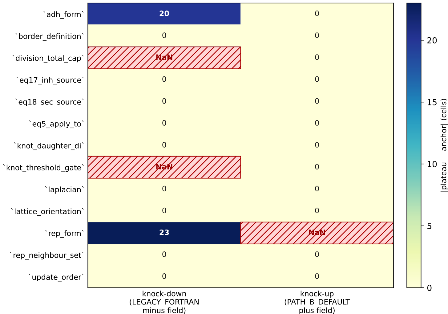
Single-field disentanglement on examples/seal.txt (absolute cell-count delta from anchor)
