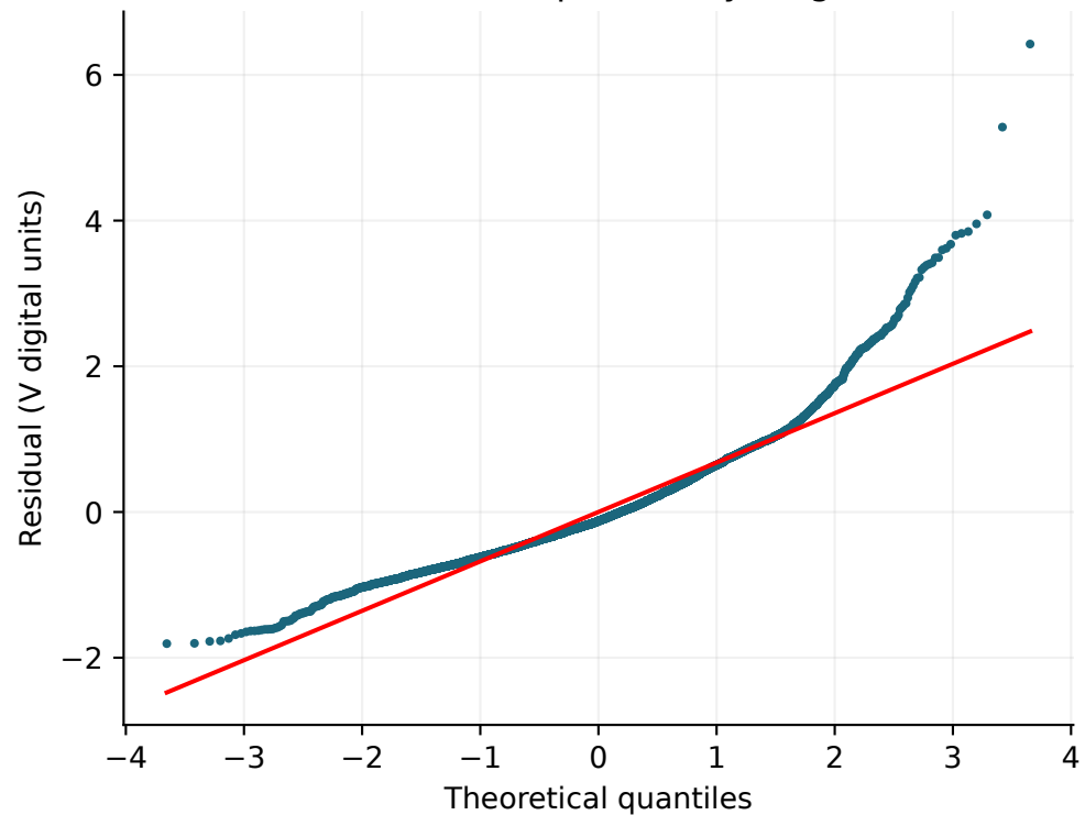
Residual normal-probability diagnostic
