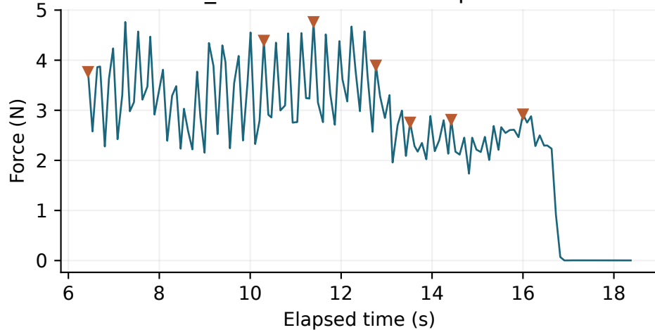
R9_TEST7: force-defined presses
