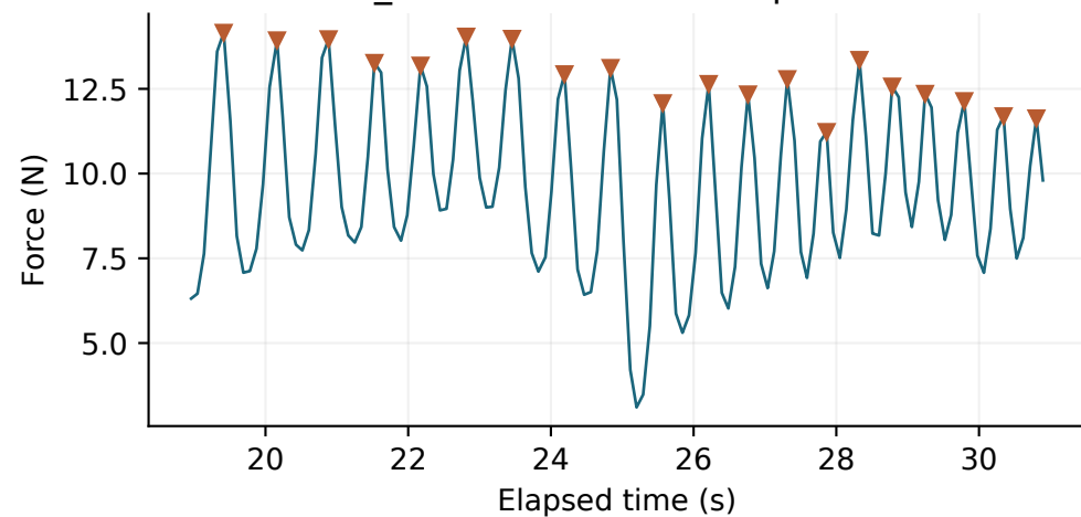
R5_TEST4: force-defined presses
