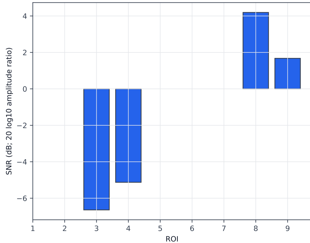
Manual contact SNR
