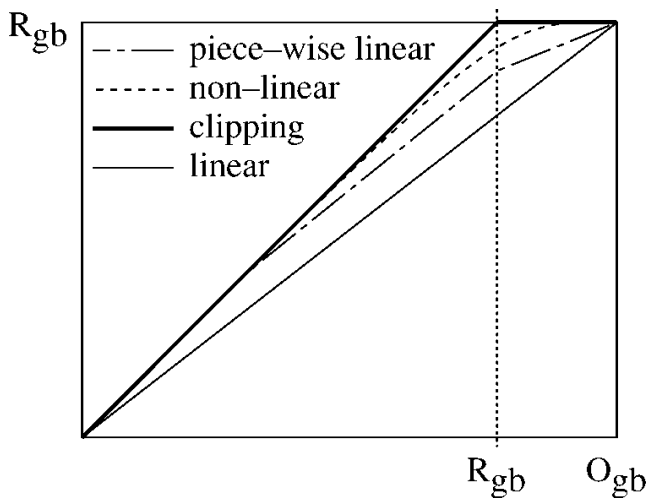
Figure 3. Gamut clipping and compression along a given line ( O_{gb} and R_{gb} represent of the original and reproduction gamut boundary respectively).
