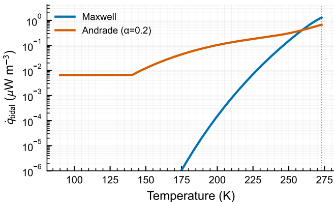
(a) Dissipation vs temperature
