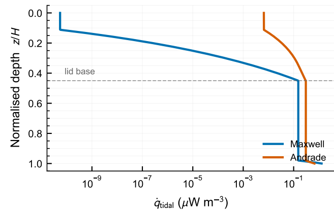
(c) Depth profile ( H = 25 km)
