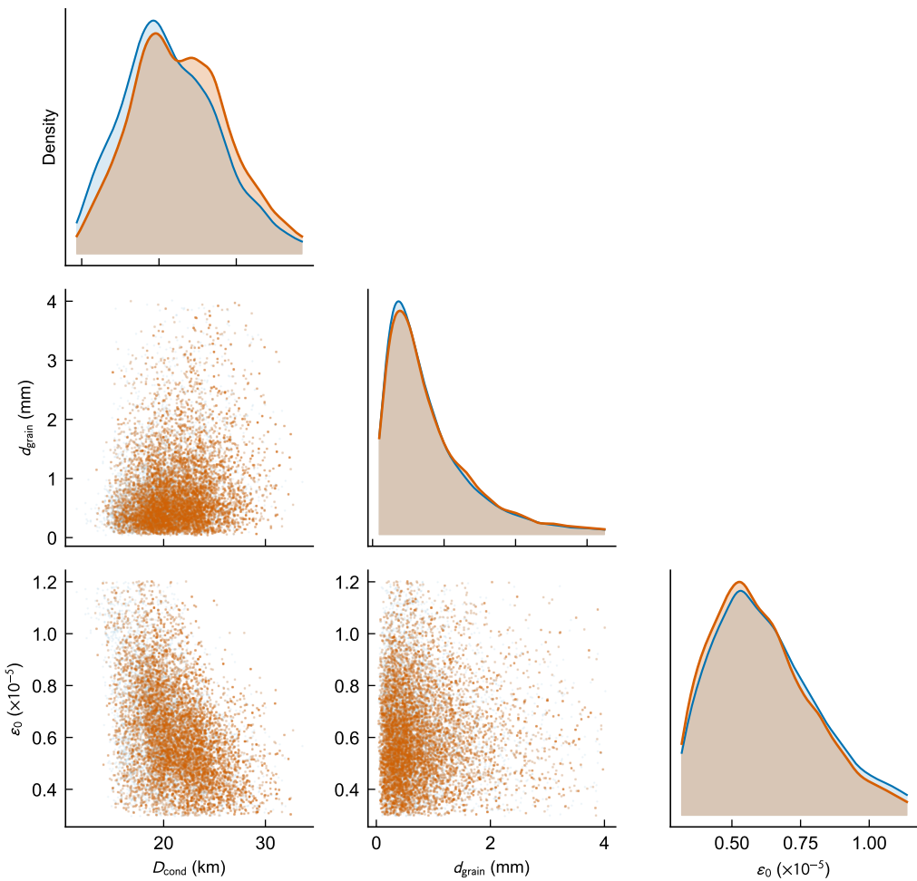
Corner plot — eq_baseline_A (ESS = 9552)
