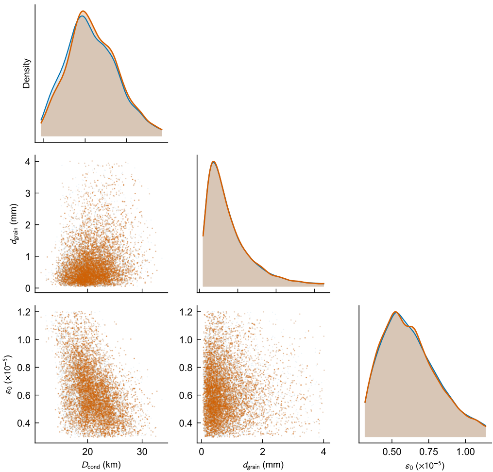
Corner plot — eq_baseline_B (ESS = 9916)
