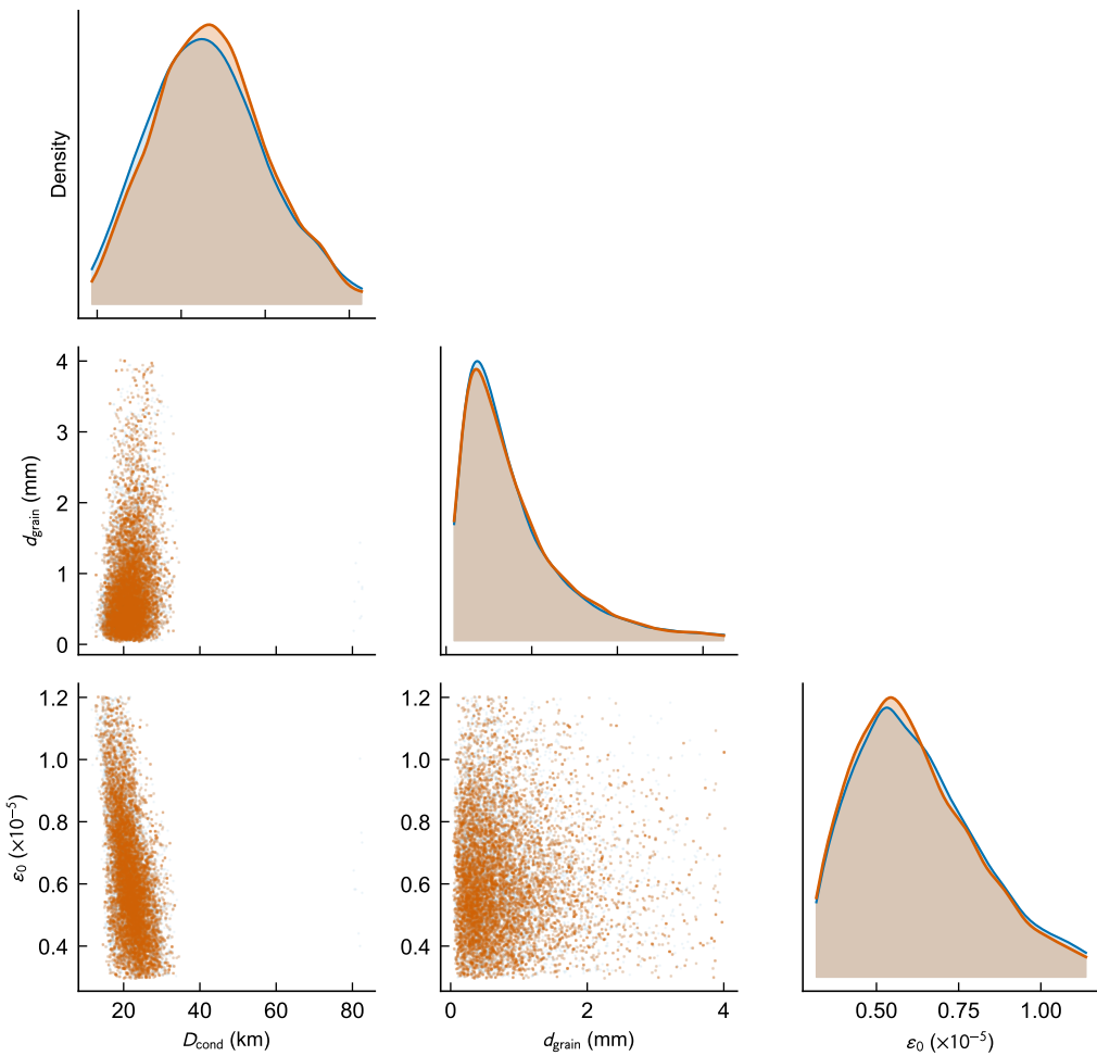
Corner plot — eq_depleted_B (ESS = 9911)
