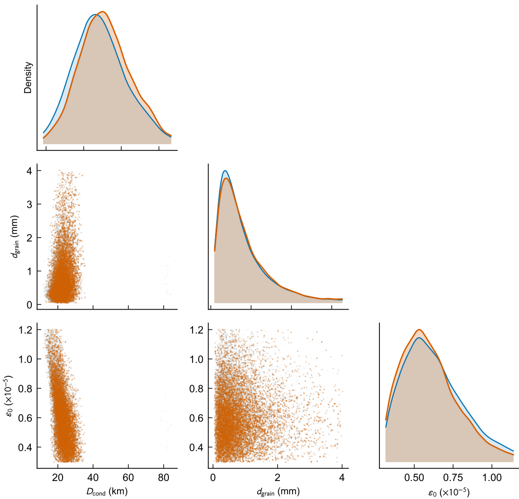
Corner plot — eq_depleted_strong_A (ESS = 14403)
