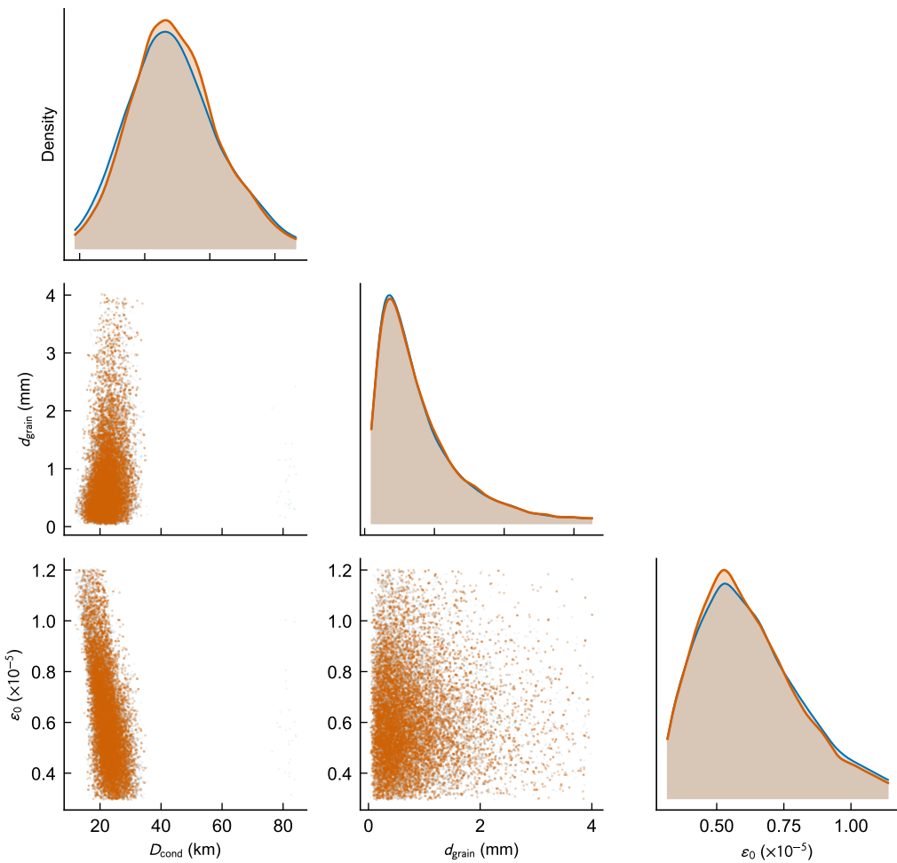
Corner plot — eq_depleted_strong_B (ESS = 14868)
