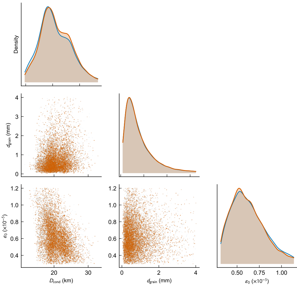
Corner plot — eq_moderate_B (ESS = 9921)
