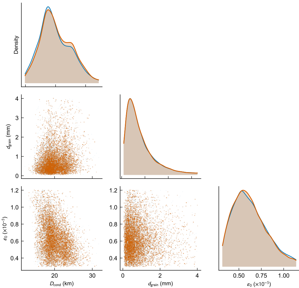
Corner plot — eq_strong_B (ESS = 9921)
