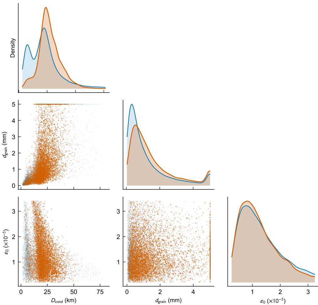
Corner plot — Model A 29 \pm 10 km (ESS = 10475)
