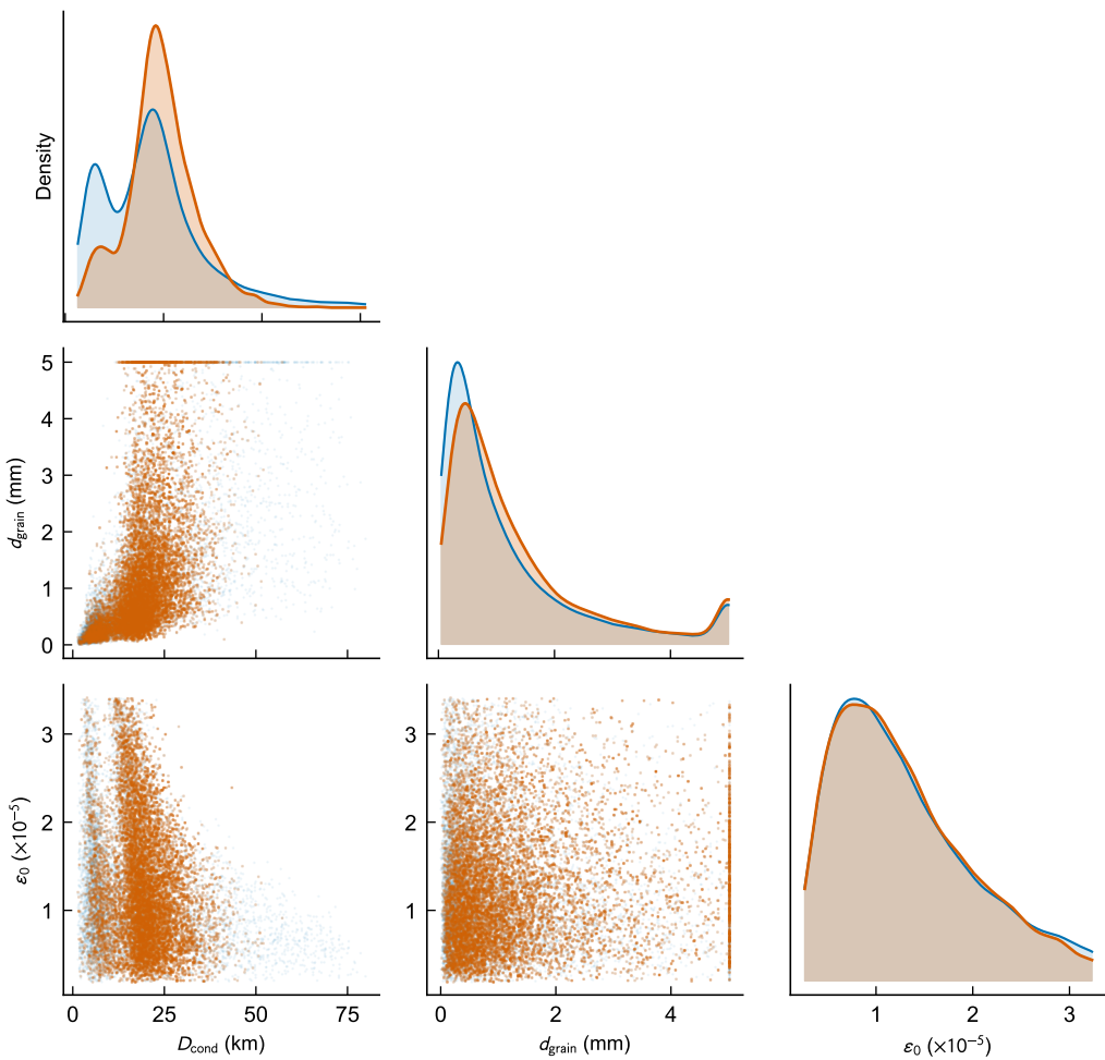
Corner plot — Model B 24±10 km (ESS = 12019)
