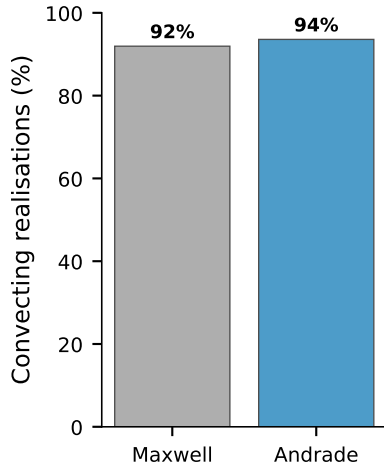
(c) Convective fraction
