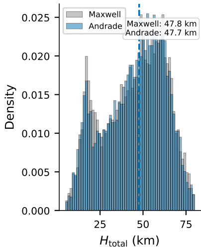
(a) Total shell thickness
