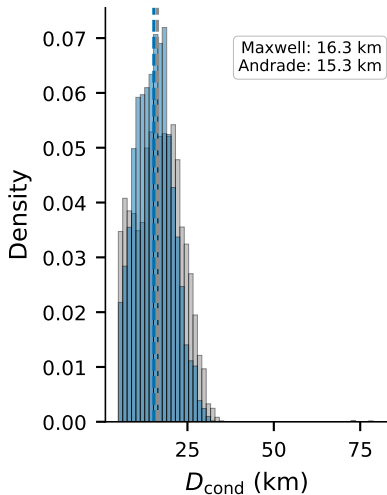
(b) Conductive lid thickness
