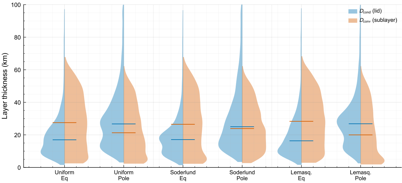
Endmember shell structure: conductive lid vs convective sublayer
