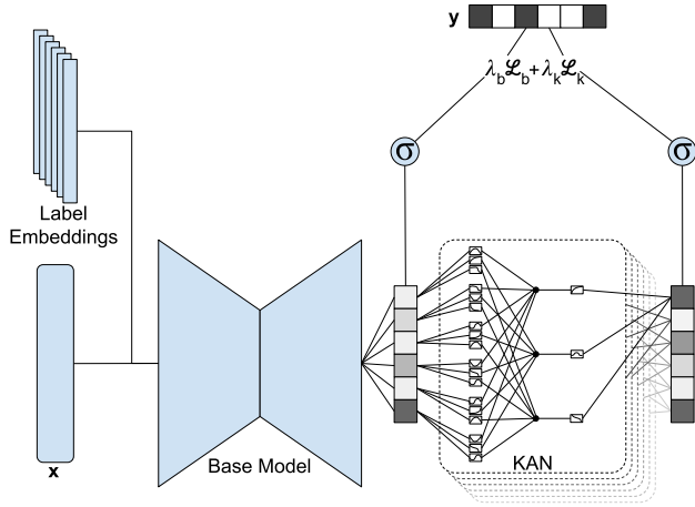
(b) LabelKAN - features are passed through a base model to get initial predictions before being input into LabelKAN.
