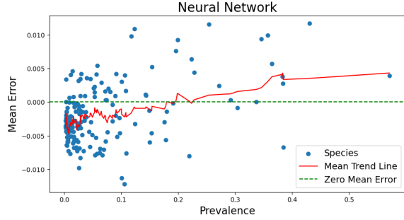
(b) Neural Network label learner error vs. species prevalence
