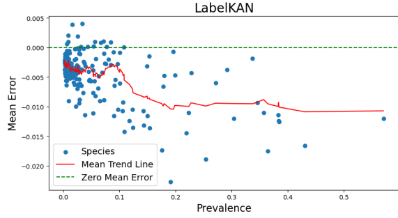
(a) LabelKAN error vs. species prevalence
