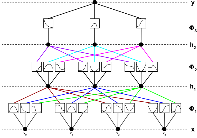
(a) Example KAN with 4 inputs, two hidden layers of width 3, and a final single output.
