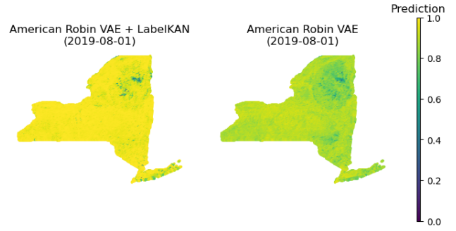
Figure 3: Predictions for the American Robin, a common species, on August 1, 2019. LabelKAN (left) results in more confident predictions (closer to the 0/1 value) across the spatial extent than the base VAE (right).
