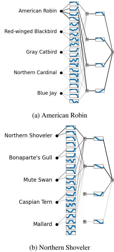
Figure 5: Subset of the learned functions and edge connection strengths from the LabelKAN model for the American Robin (top) and Northern Shoveler (bottom), the most and least prevalent species respectively, showing the top 5 contributing species for each. For the American Robin, most of the signal comes from itself, whereas for the Northern Shoveler, the signal strength from the input species logits is more distributed across co-occurring species.
