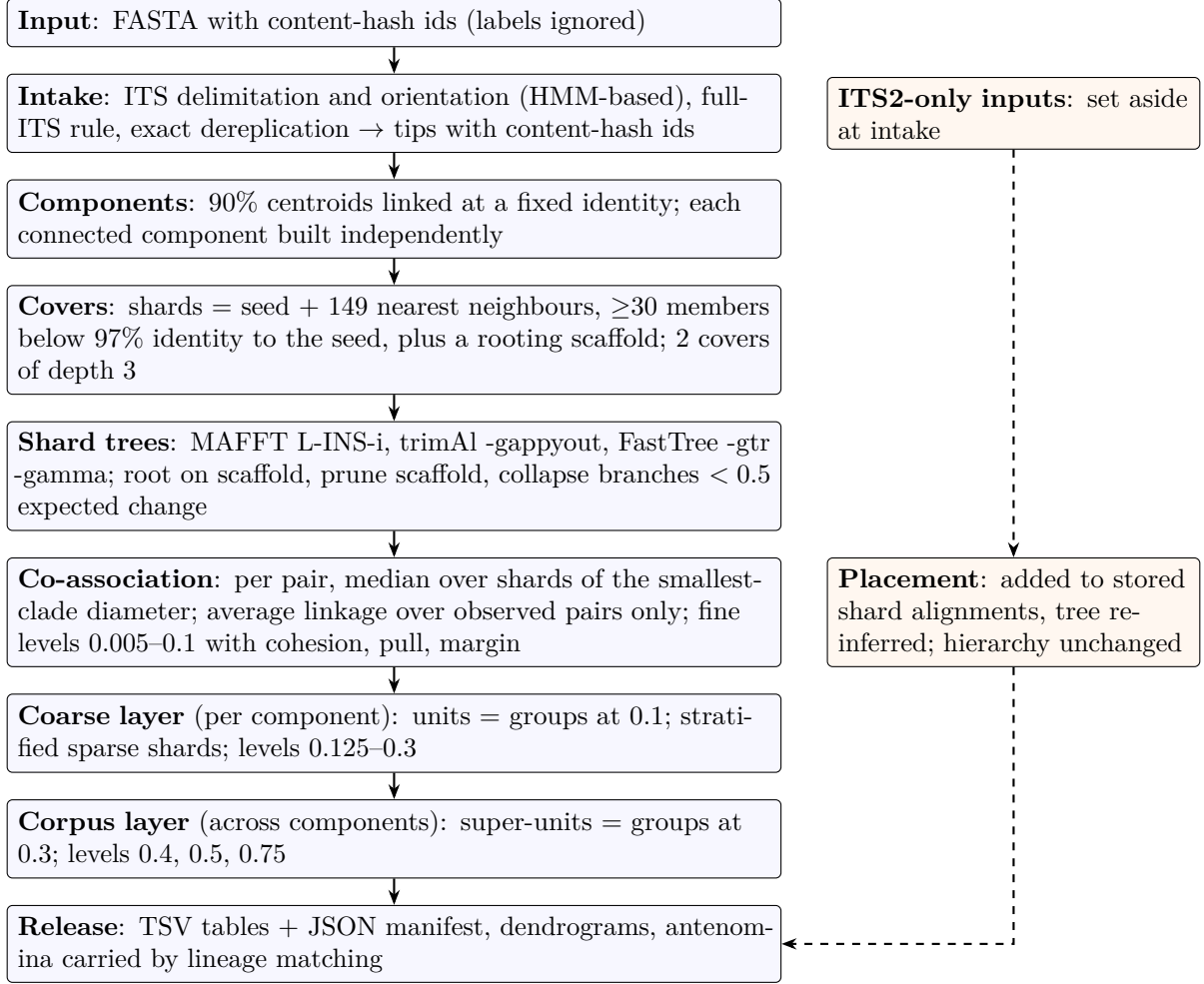
Figure 1: The seqhession pipeline. Sequence identity (vsearch) is used only to decide what is sampled together: components, shard neighbourhoods, the scaffold and candidate shards for placement. Every grouping decision is made from tree distances in the shard trees.
