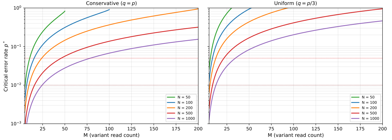
Figure 2: Critical error rate p^* vs. variant read count M for several total read counts N ( K = 1 , L = 700 , \alpha = 0.05 ). Left: conservative model ( q = p ). Right: uniform model ( q = p/3 ).
