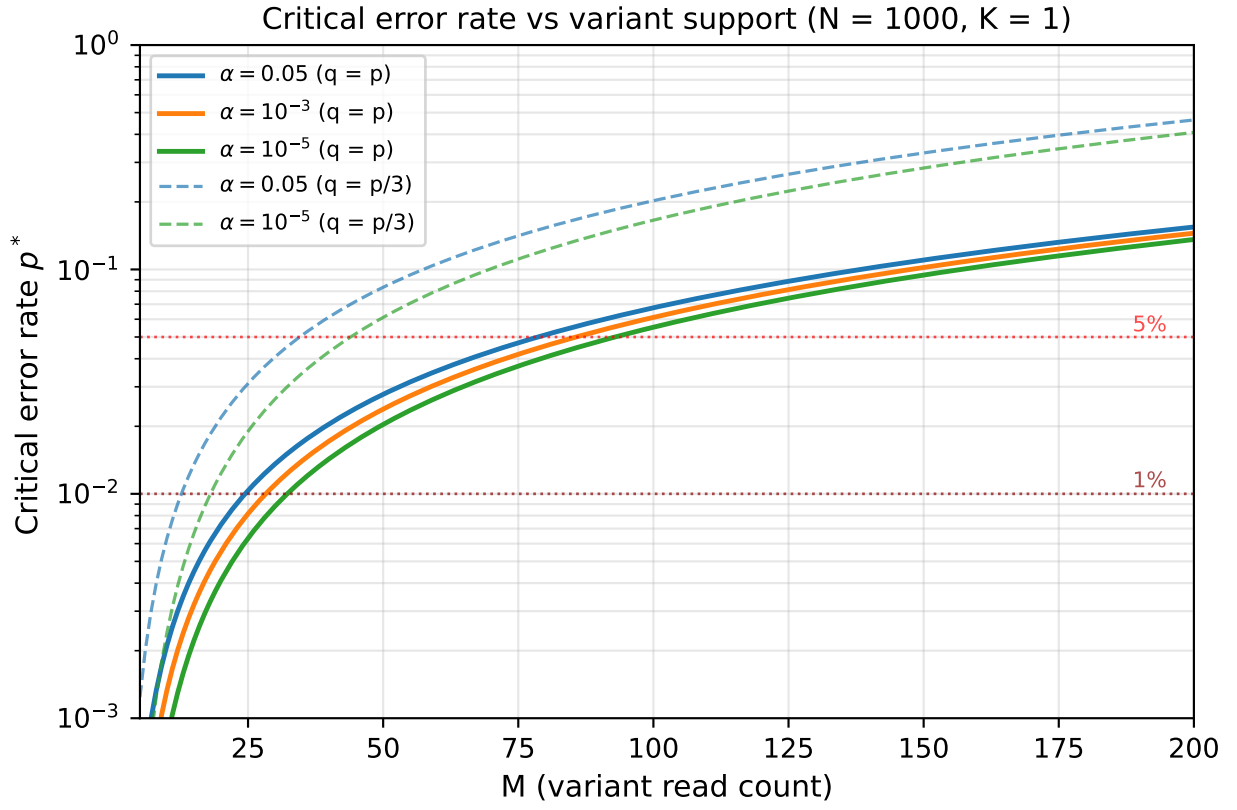
Figure 1: Critical error rate p^* vs. variant read count M at N = 1000 , K = 1 , L = 700 . Solid lines: conservative model ( q = p ) at three significance levels. Dashed lines: uniform model ( q = p/3 ) at \alpha = 0.05 and \alpha = 10^{-5} .
