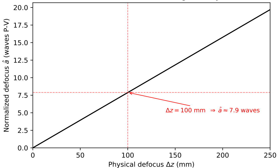
Defocus unit conversion — SEAL geometry (F/49.4)
