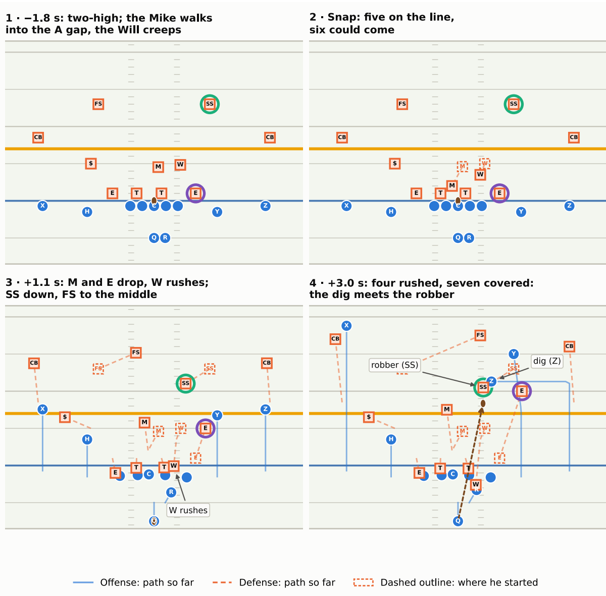
Figure 5: The double lie (simulated, BDB-format tracking generated by gridiron; illustrative, not a specific Seahawks call). Third-and-7. 1: before the snap the defense shows two-high, and the Mike (M) walks up into the left A gap: with the four linemen that is five on the line, and the Will (W) creeps to about three and a half yards, so six could rush. The nickel ($) could just as well be Seattle's third safety; the picture is the same. 2: at the snap nothing has moved in the secondary. 3: the lie about the rush. The Mike backs out to the hook and the right edge (E, purple ring) drops to wall off the tight end (Y), while the Will rushes through the right B gap and the back steps up to block him. Four rush: one of them (W) a player the protection had to guess about, and two of the six it counted (M, E) are in coverage. The lie about the coverage: the strong safety (SS, green ring) comes down to the hole, the short middle at about 10 yards, and the free safety runs to the deep middle, so two-high has become Cover 3 with a robber. 4: the dropped edge has carried Y up the seam until the free safety, shaded to that side, takes him. The quarterback, who saw an open middle before the snap and a blitz threat to his left, throws the dig to Z; it arrives where the robber is. Dashed outlines show where the defenders started.
