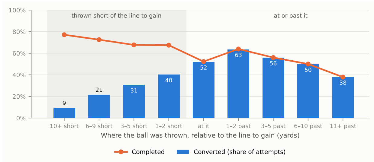
Figure 3: Where third-down passes were aimed, and what happened. Each bar is the share of attempts that converted, grouped by how far past (or short of) the line to gain the ball was thrown (air yards minus yards to go); the line is the completion rate for the same throws. Throws short of the line are caught more often but convert rarely, because the receiver still has to run for the rest; throws one or two yards past it convert most often; deeper throws are completed, and so convert, less often. Third-down aimed passes (sacks, scrambles and throwaways without a charted depth excluded), NFL regular seasons 2021–2025. Source: nflverse play-by-play.
