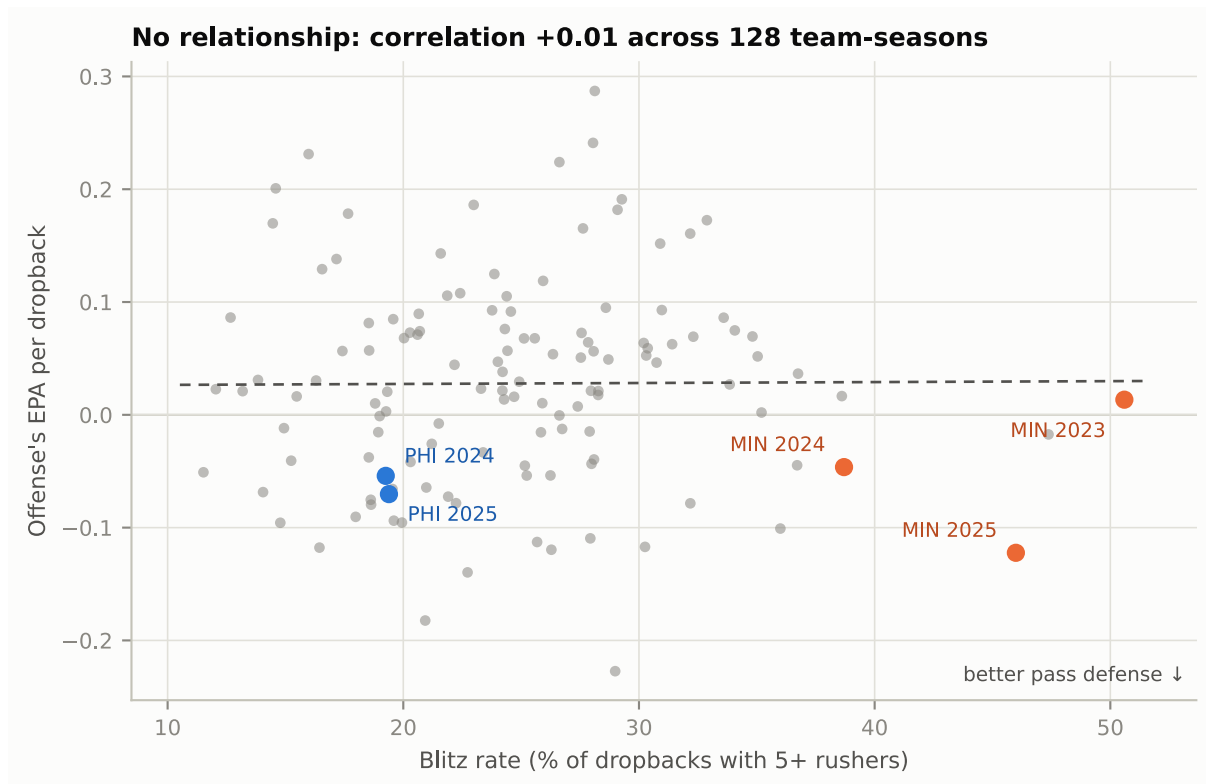
Figure 7: Blitz rate against pass defense, every team-season from 2022 to 2025 (FTN charting; regular season; a blitz is five or more rushers). The horizontal axis is the share of opponents' dropbacks on which the defense blitzed; the vertical axis is the offense's average EPA per dropback (lower is better for the defense). There is no slope: heavy-blitzing and light-blitzing defenses have done equally well and equally badly. Brian Flores's Vikings (orange) led the league in blitz rate in 2023, 2024 and 2025 and ranked 15th, 3rd and 2nd in EPA per dropback allowed; Vic Fangio's Eagles (blue) blitzed among the least in 2024 and 2025 and ranked 2nd and 7th. Coaches choose their blitz rates, so this is an association, not an experiment.
