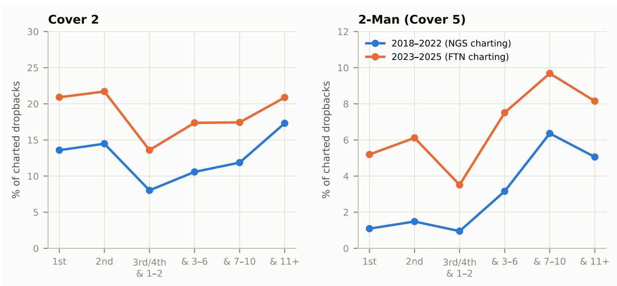
Figure 8: When NFL defenses call Cover 2 and 2-Man, by down and distance (share of charted regular-season dropbacks). Left, Cover 2 (zone): fairly steady on early downs and third-and-long, least common on third-and-short, where the offense needs only a yard or two and squat corners and deep safeties are the wrong tools. Right, 2-Man: rare on early downs and peaking on third-and-7 or more, where the defense must cover the receivers at the sticks and keep two safeties deep. The charting source changed after 2022 and FTN labels both coverages more often than Next Gen Stats did, so compare the shapes, not the levels.
